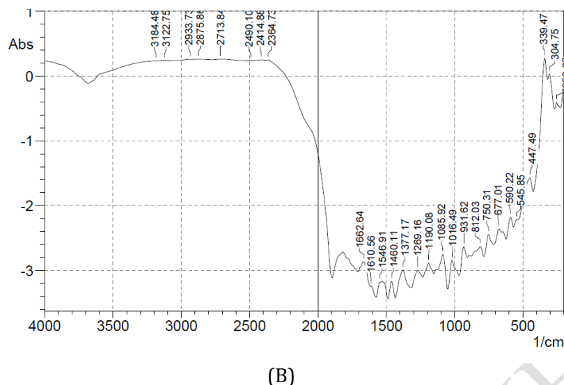
Figure 2. The FT-IR measurements spectra of Ag nanoparticles prepared by different peel extract by (A) banana extraction (B) Orange extraction.
