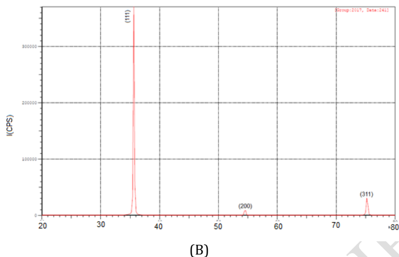
Figure 1. presents XRD diffraction of Ag NPs prepared by (A) banana extraction (B) Orange extraction.
