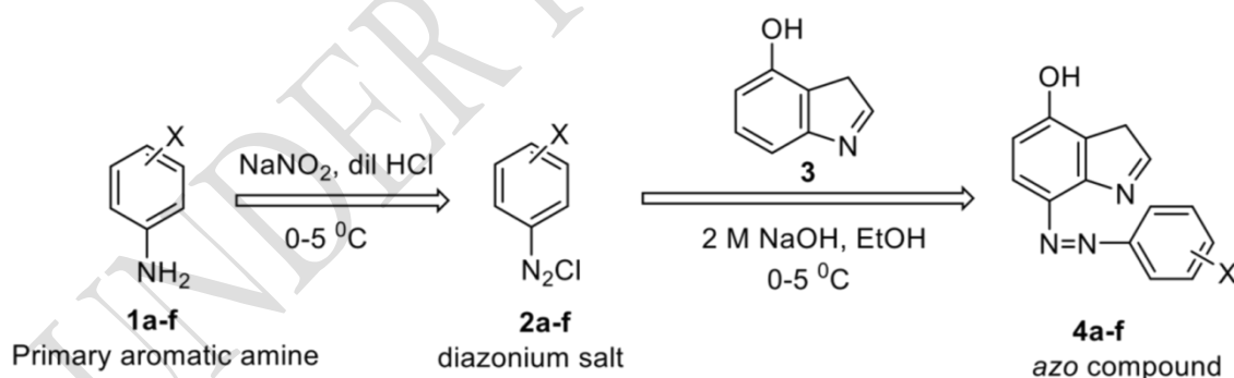
Scheme 1: General scheme for the synthesis of the azo compounds 4a-f ; 4a ( \text{X}=\text{p-NO}_2 ), 4b ( \text{X}=\text{m-NO}_2 ), 4c ( \text{X}=\text{o-NO}_2 ), 4d ( \text{X}=\text{2-Cl-p-NO}_2 ), 4e ( \text{X}=\text{p-COCH}_3 ), 4f ( \text{X}=\text{p-COOH} ): o , m and p represent ortho , meta and para substitution respectively.
