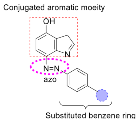
Fig. 1: Scaffold design for azo compounds 4a-f
