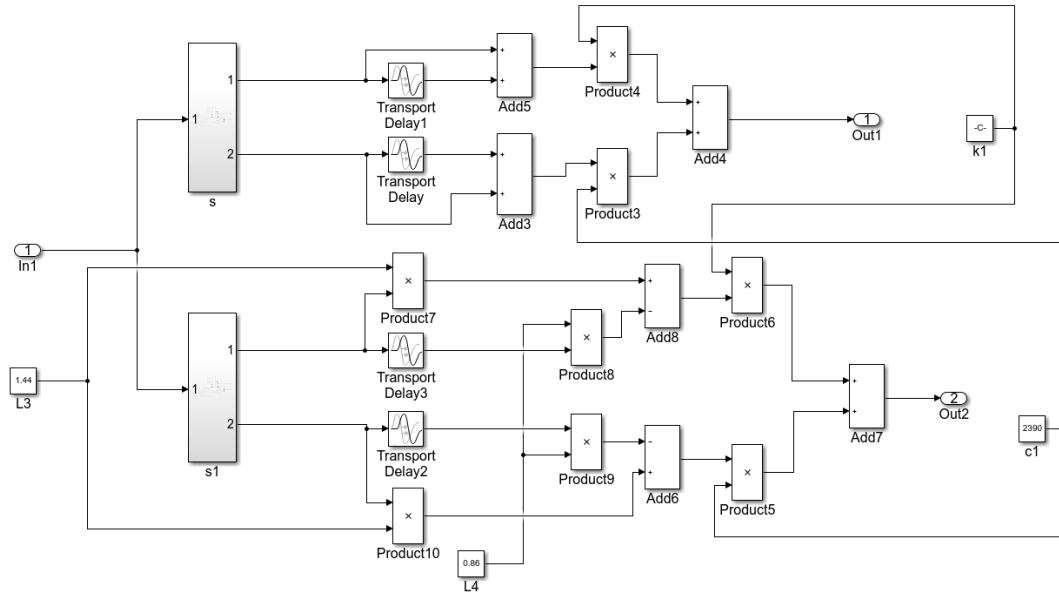
Fig. 4. Subsystem diagram of vector F
