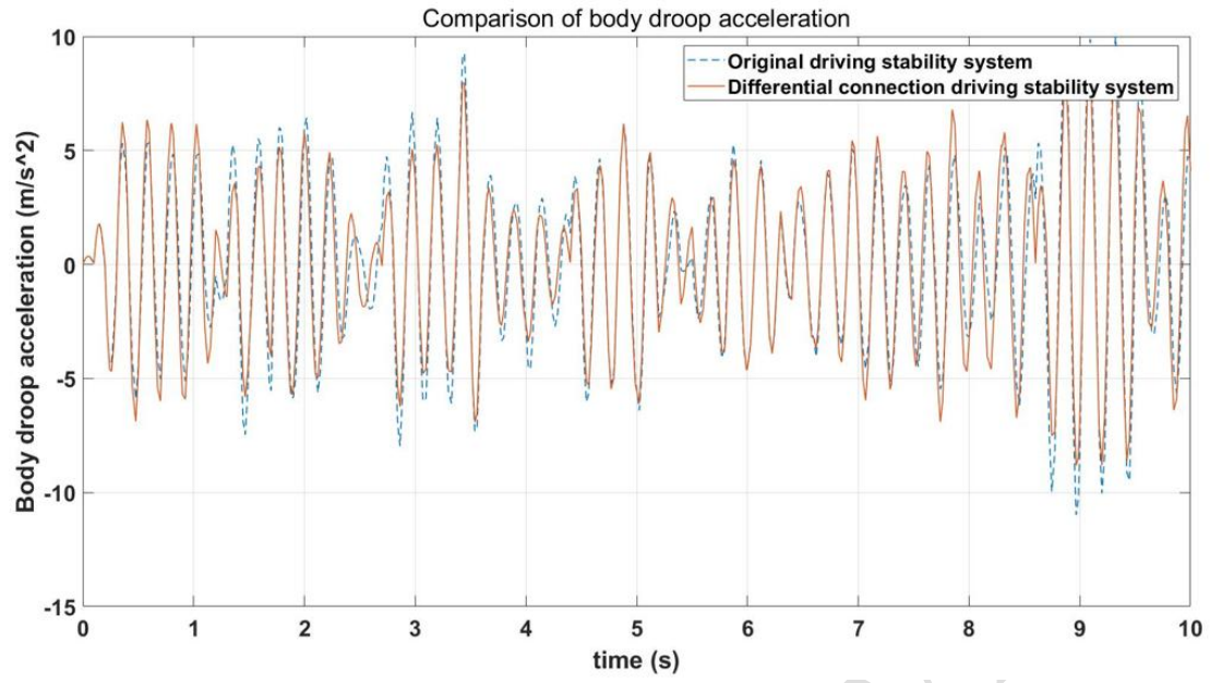
Fig. 5. Comparison of simulation results of body vertical acceleration
