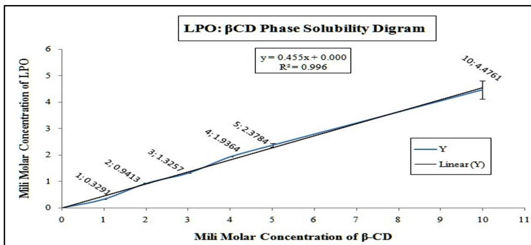
Fig. 2: Phase solubility analysis of LPO with β-CD
