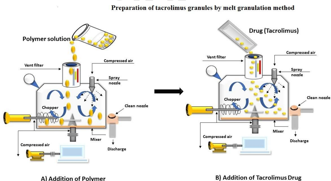
Image 1 : Preparation of tacrolimus granules by melt granulation method
