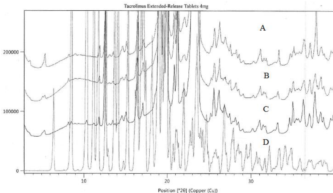
Fig 6: XRD thermogram of (A) Placebo, (B) tacrolimus extended release tablets initial, (C) Tacrolimus extended release tablets 6 months 40°C/75%RH and (D) tacrolimus drug substance
