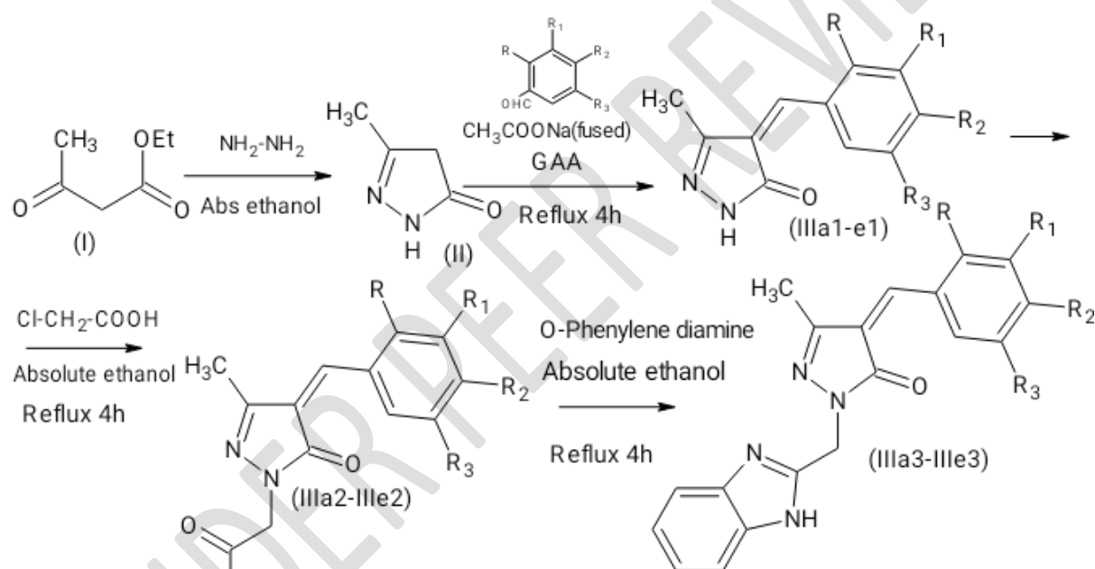
Fig. 1: Synthesis Scheme
