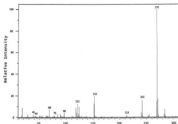
III-d (Mass spectra)
