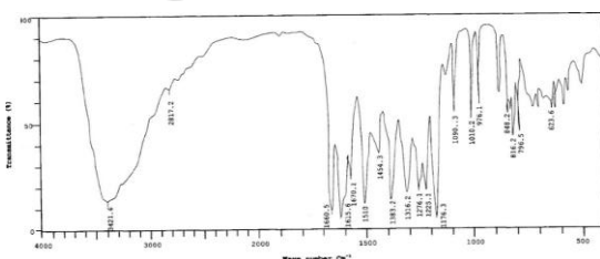
Fig 1:Spectral data of compound I I-a (IR spectra )
