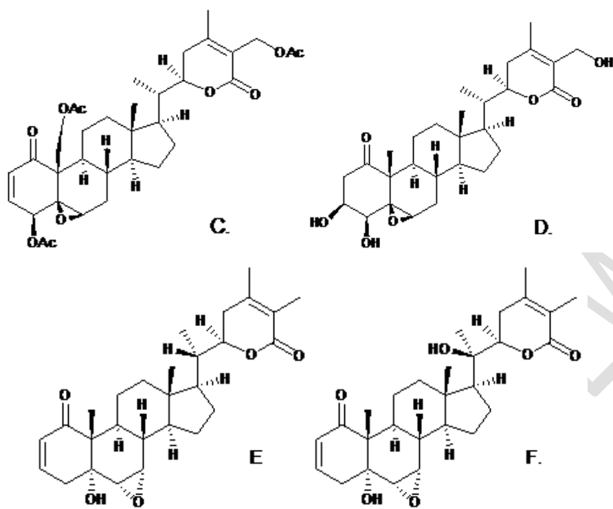
Figure 2: Structure of the Ashwagandha extract compounds from leaves, roots, stem and fruits (A) Withaferin A, (B) Withalongolide A, (C) Withaferin triacetate, (D) 2,3-Dihydro-3 \beta -methoxy Withaferin A, (E) Withanone, (F) Withanolide A [10] .
