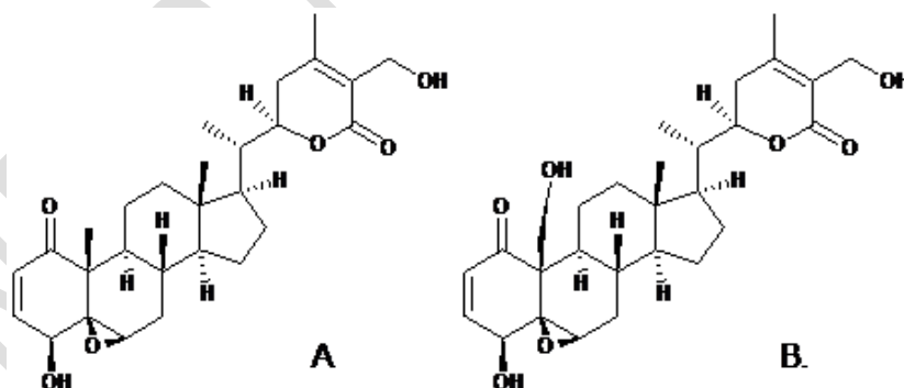
Figure 1: Ashwagandhanolide, a new compound isolated from W. Somnifera
