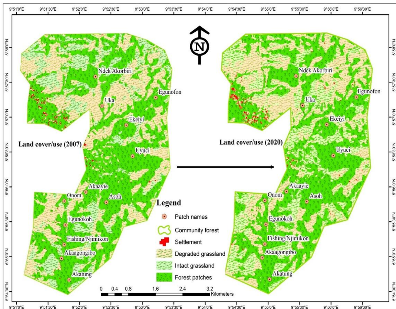
Figure 4: Land Cover/Use for 2007 and 2020
