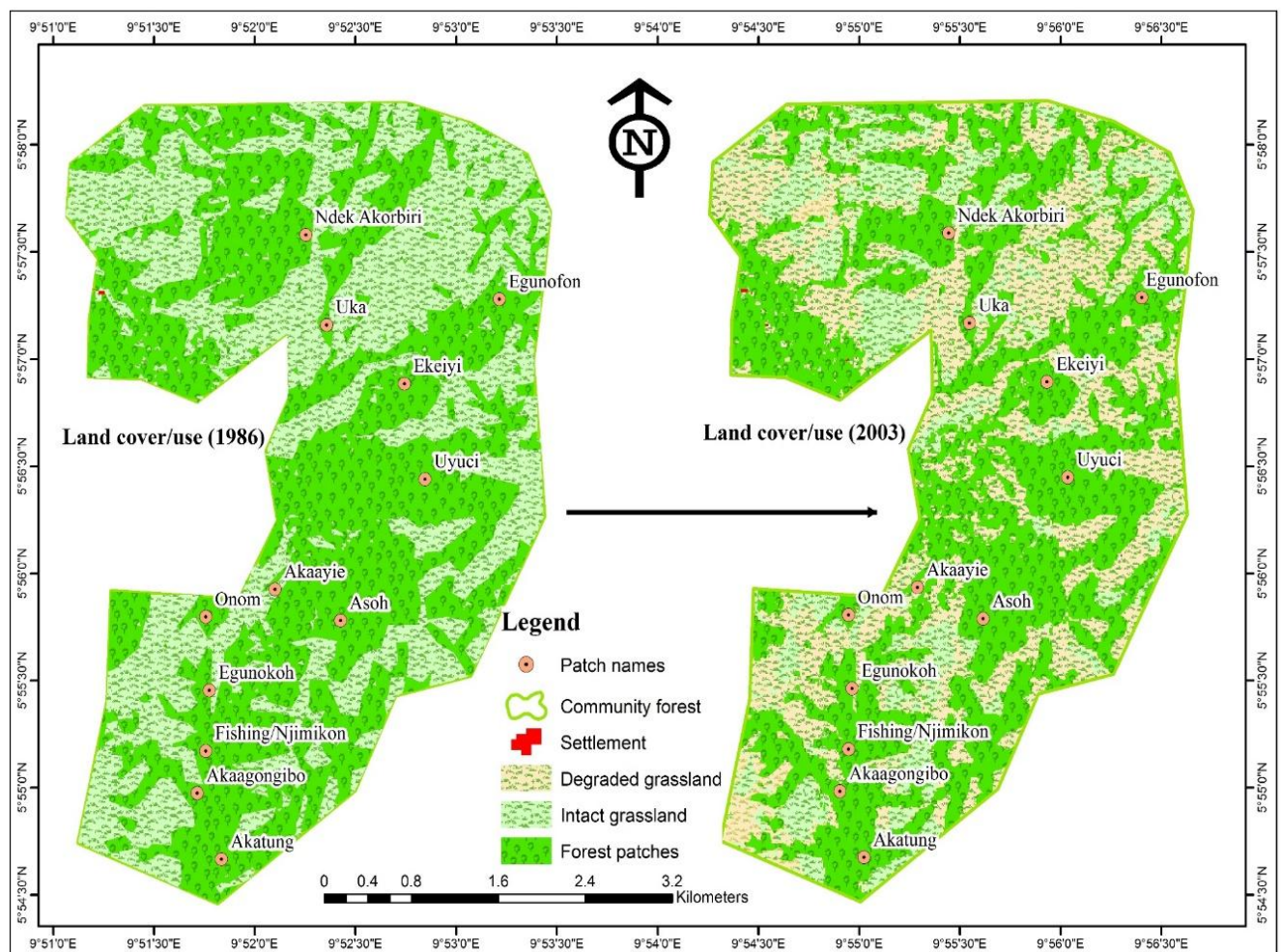
Figure 3: Land cover/use for 1986 and 2003
