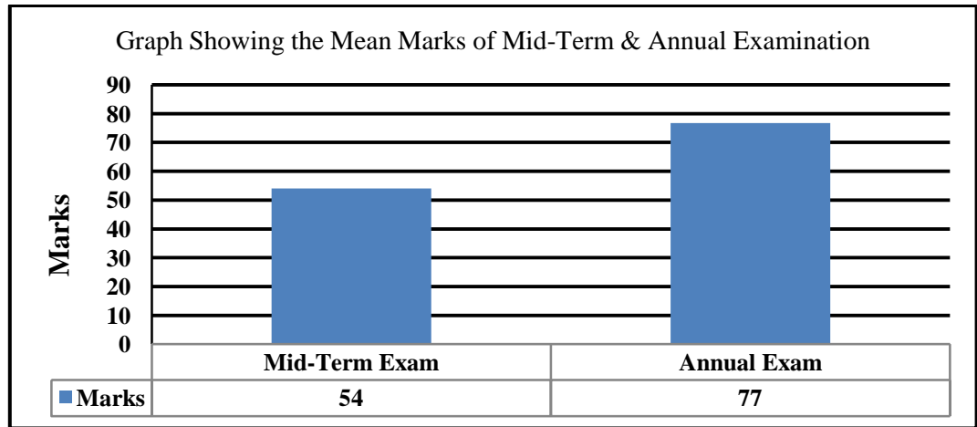
Figure 2: Comparison of learning achievement of mid-term and annual exam
