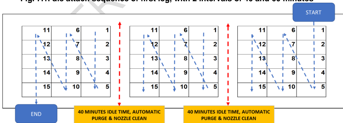
Fig. 7.2. die attach sequence of first leg, with 2 intervals of 40 and 60 minutes; automatic purge and pre dispense activated
