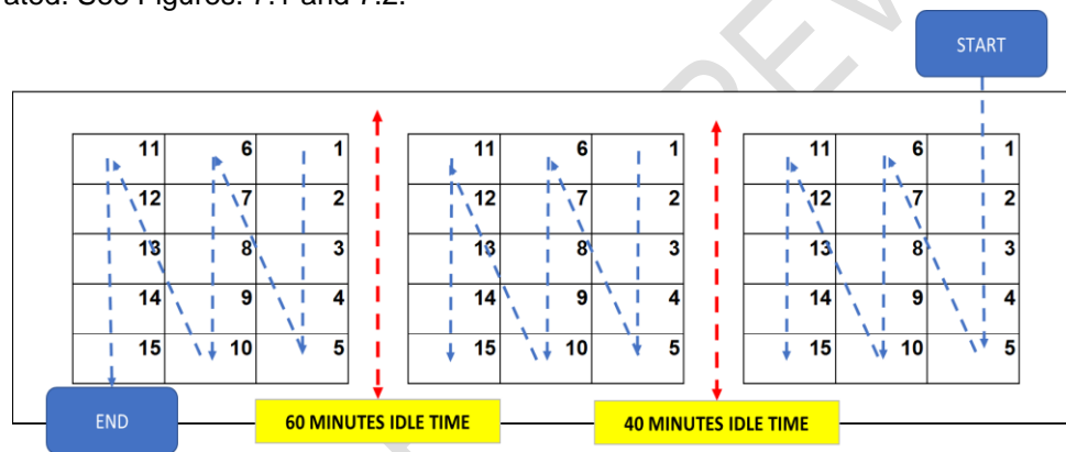
Fig. 7.1. die attach sequence of first leg, with 2 intervals of 40 and 60 minutes
