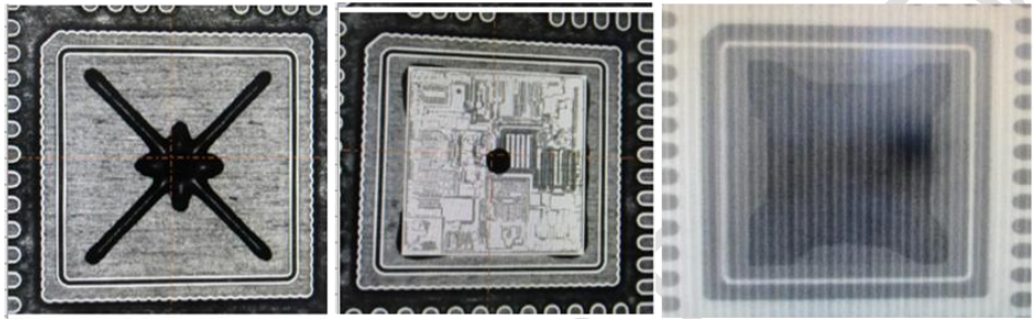
Fig. 4. Ideal and insufficient epoxy coverage shown on four sides of die
