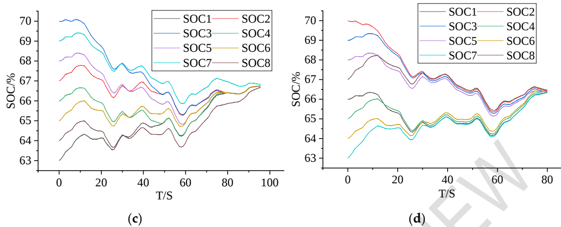
Fig. 12. Different initial SOC equalisation results
