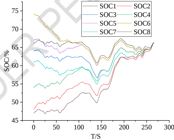
Fig. 8. Equilibrium process SOC changes
