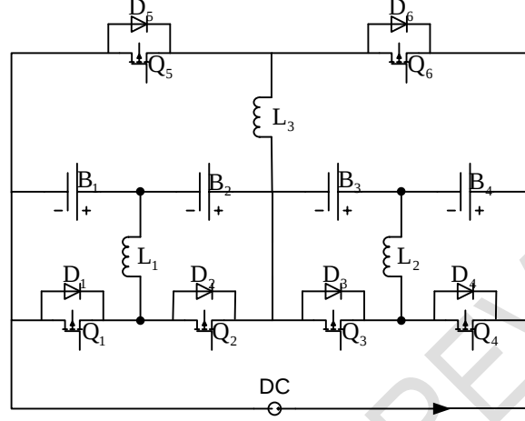
Fig. 2. Battery pack equalization circuit
