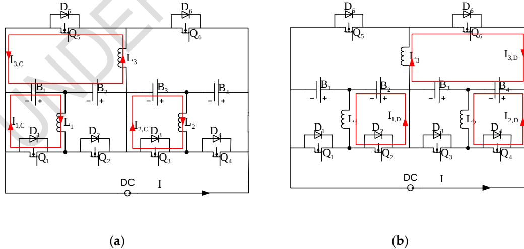
Fig. 3. (a) Schematic of first stage of charge equalization, (b) Schematic of the second stage of charge equalization
