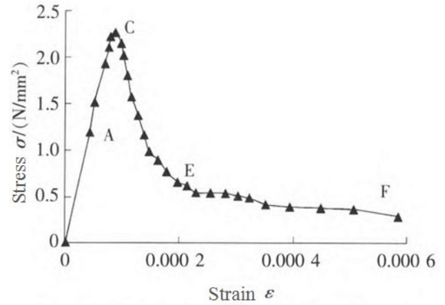
Fig.3 The Tensile stress-strain curve of concrete
