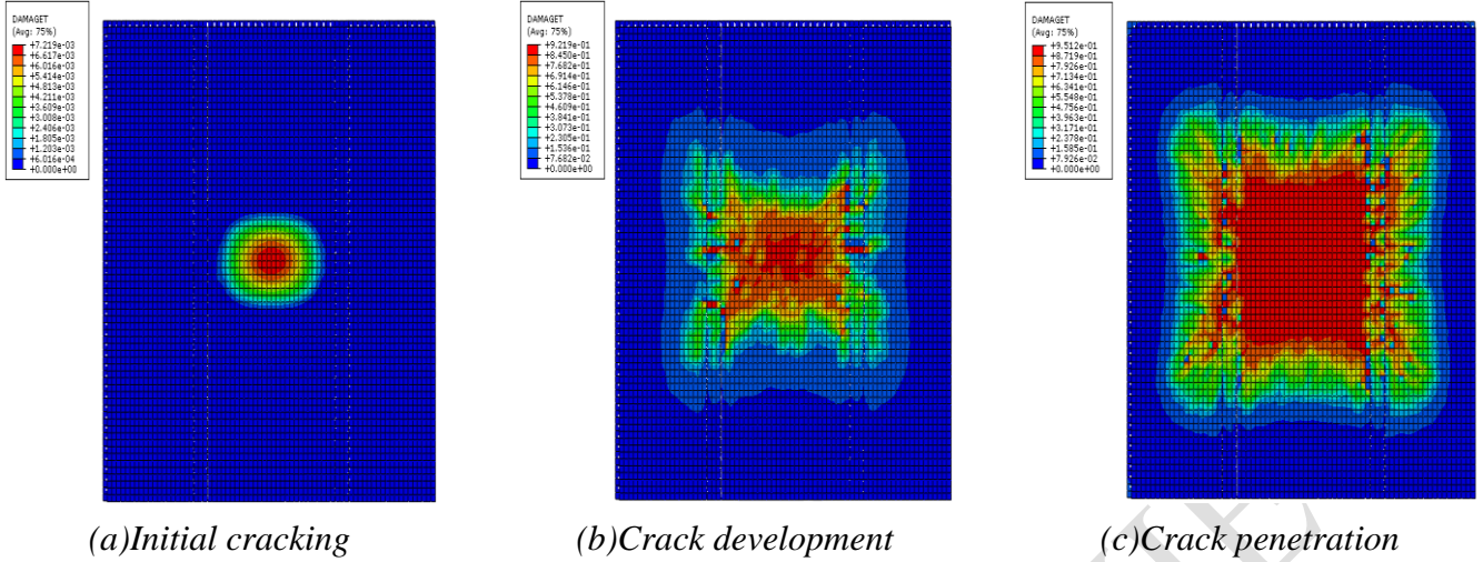
Fig.8 Damage distribution in different stress stages of model B
