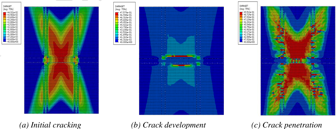
Fig.9 Damage distribution in different stress stages of model C
