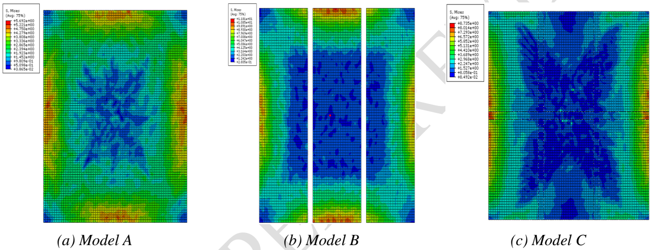
Fig.10 Stress distribution of three kinds of slabs in cracks penetration stage
