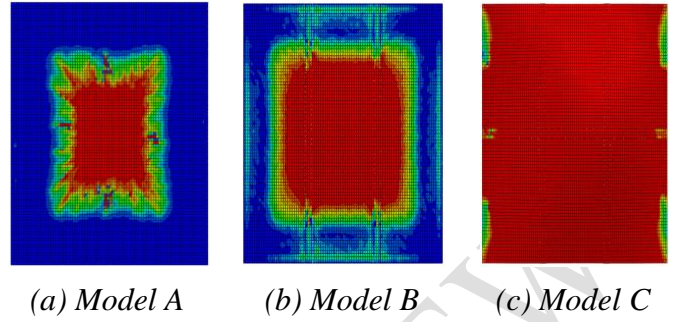
Fig.6 Plastic damage of the bottom of slab under ultimate load
