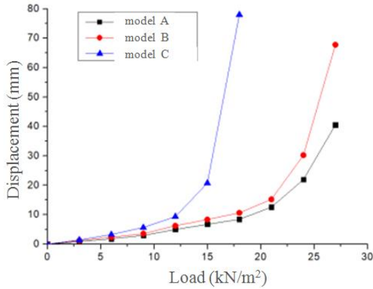
Fig.5 The midspan load-displacement curve of three kinds of slabs
