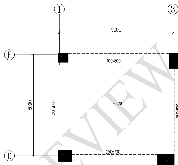
Fig.1 The large-span slab of a project
