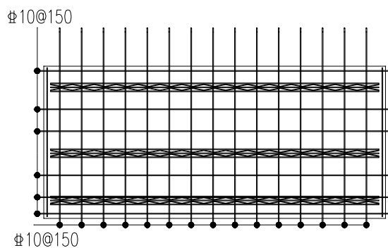
Fig.2 The reinforcement drawing of composite slab
