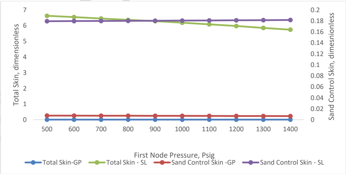
Figure 4: Effect of First Node Pressure on Skin Development
