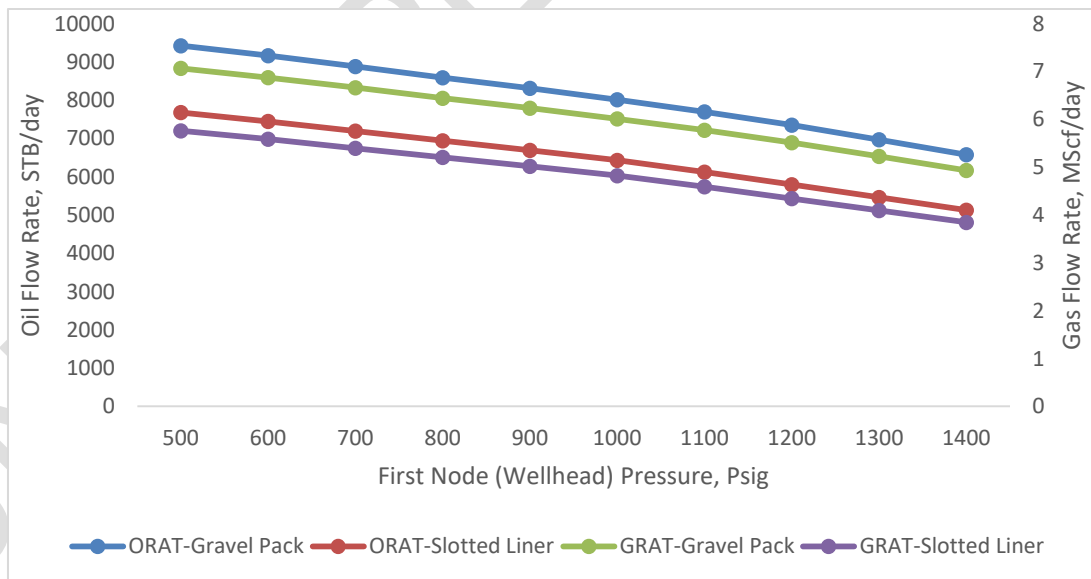
Figure 3: Effect of Wellhead Pressure on Oil and Gas Production Rates
