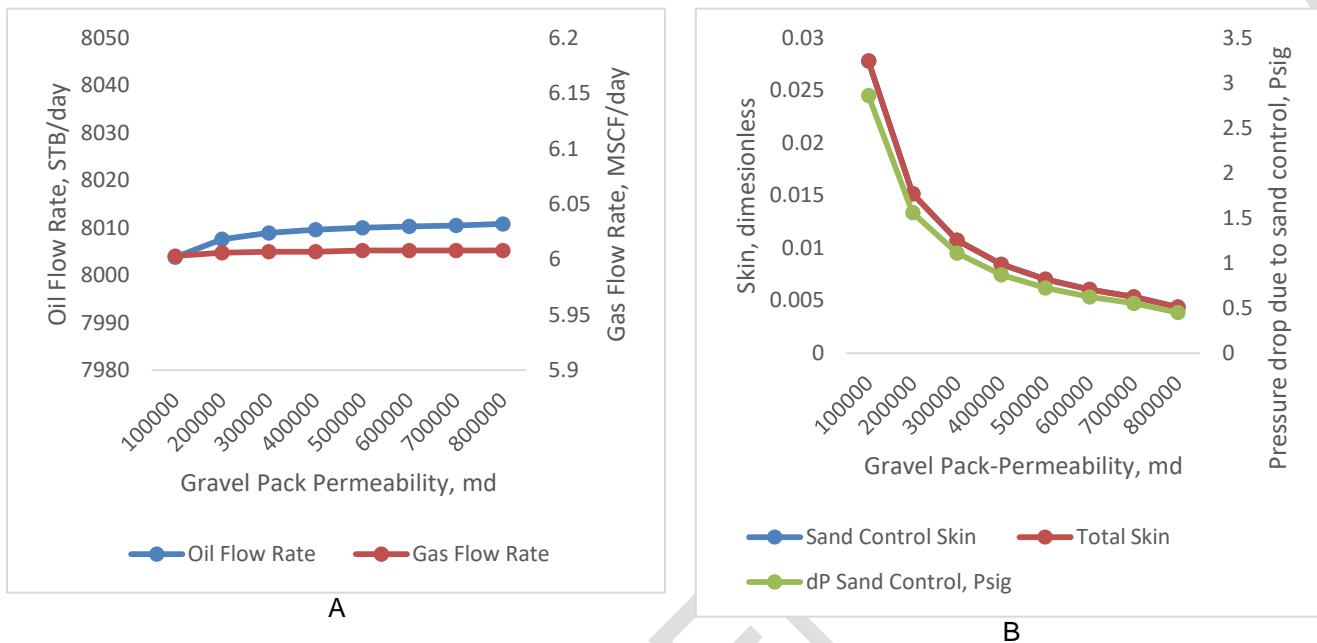
Figure 6: Effect of GP Permeability on: (A) Production Rates and (B) Skin Development
