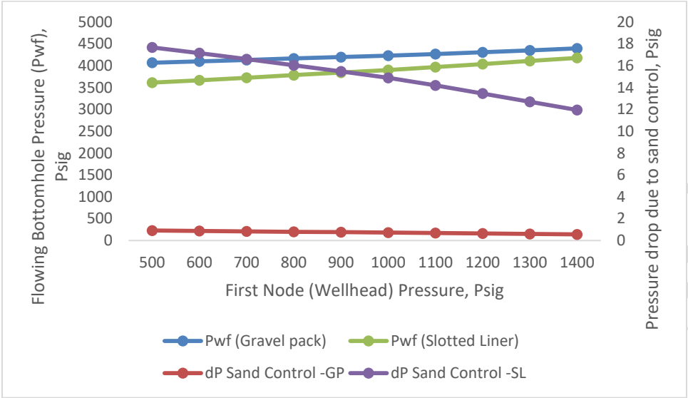
Figure 4 Effect of First Node Pressure on Pwf and ΔP Sand Control
