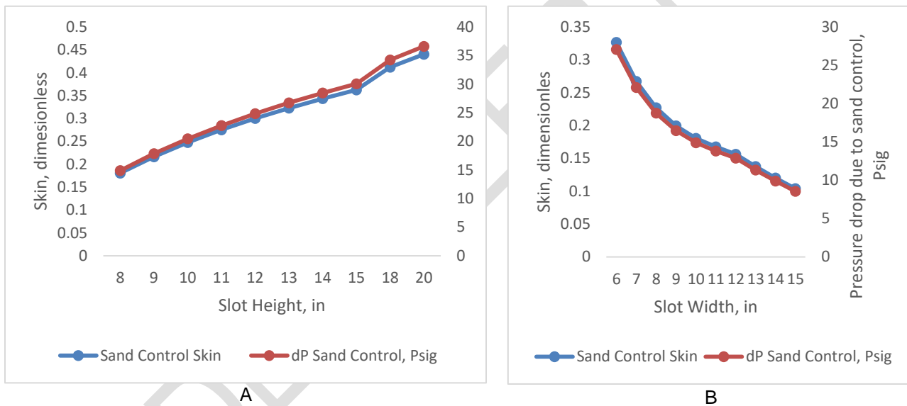
Figure 8: Effect of Slot Dimensions on Production Rates: (A) Slot Height and (B) Slot Width
