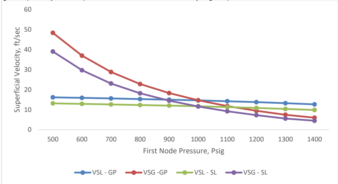
Figure 6: Effect of First Node Pressure on Superficial Fluid Velocities
