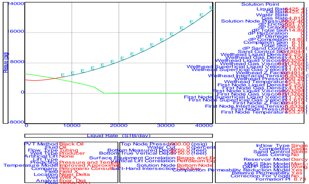
Figure 2: IPR-VLP Plot of Slotted Liner Option – Base Case
