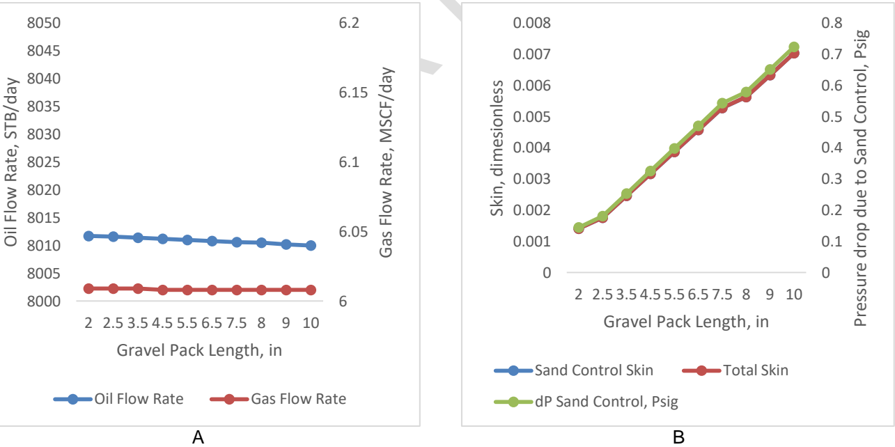
Figure 5: Effect of GP Length on: (A) Production Rates and (B) Skin Development.
