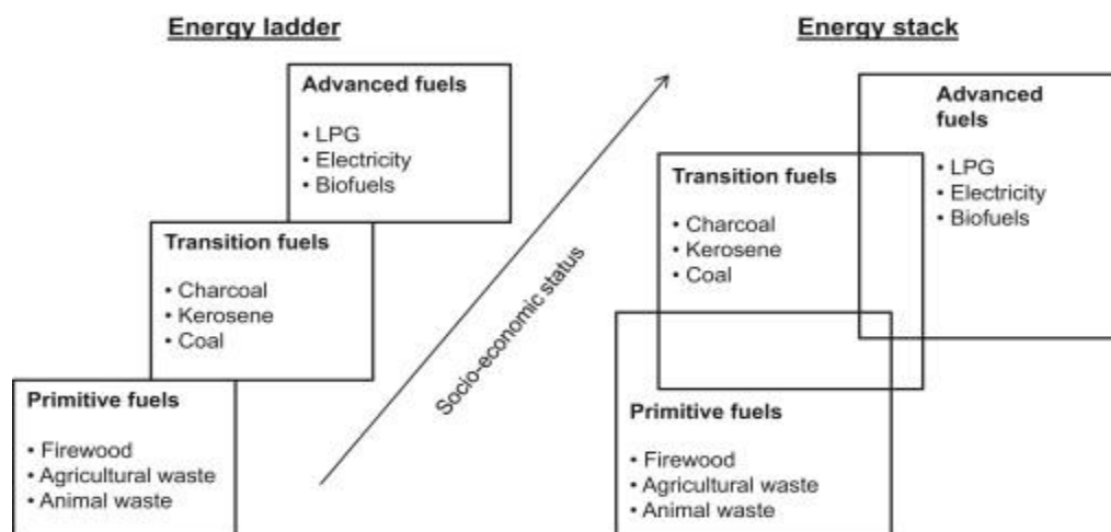
Figure 1: Energy ladder and energy stack models
