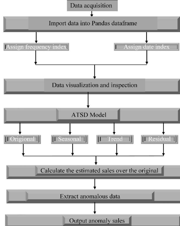
Fig. 1. Sales anomaly detection process
