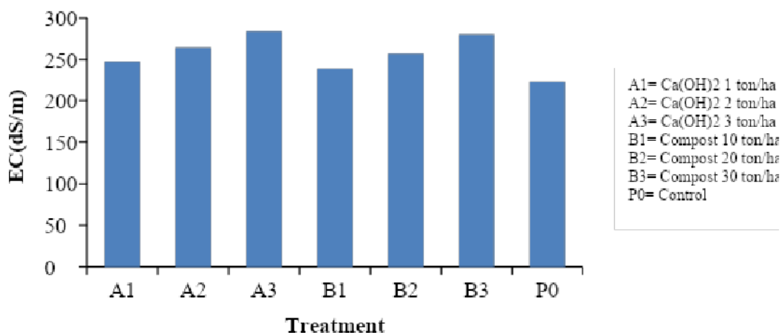
Figure 2. Soil electrical conductivity during incubation
