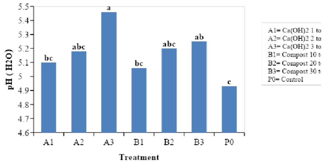
Figure 1. Effect of compost and \text{Ca}(\text{OH})_2 on soil pH at week 8
