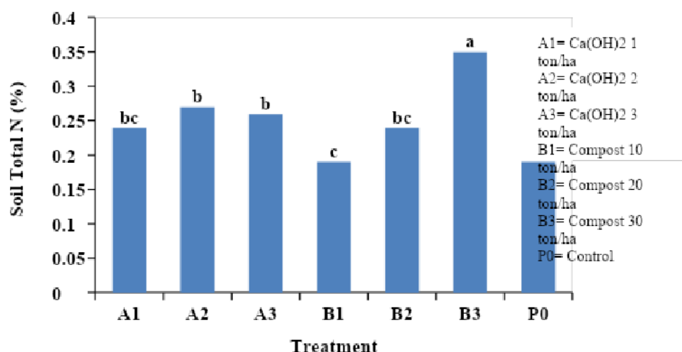
Figure 5. Effect of \text{Ca(OH)}_2 and Compost on total soil N
