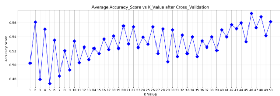
Fig. 3.3 Line graph of average accuracy score with K- values after cross validation
