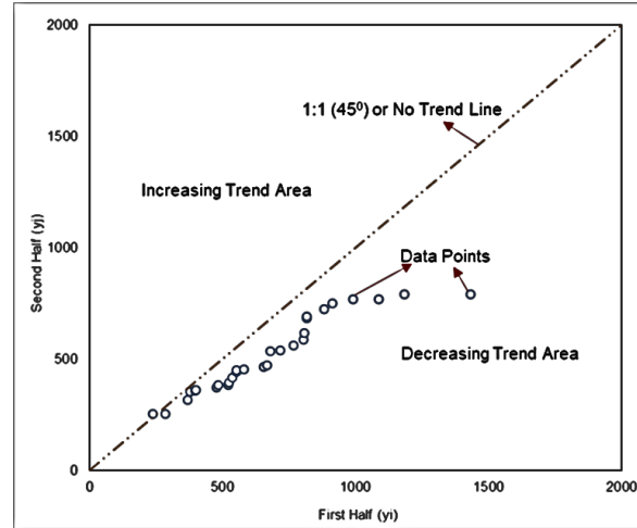
Figure 3: Trend in time-series data by a visual interpretation by ITA method.
