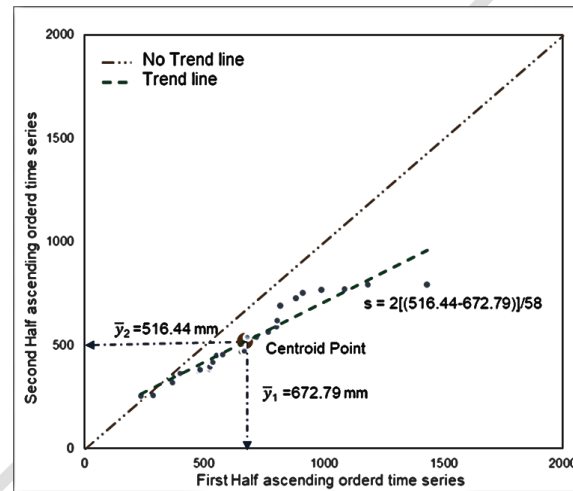
Figure 4: Slope analysis by the ITA method.
