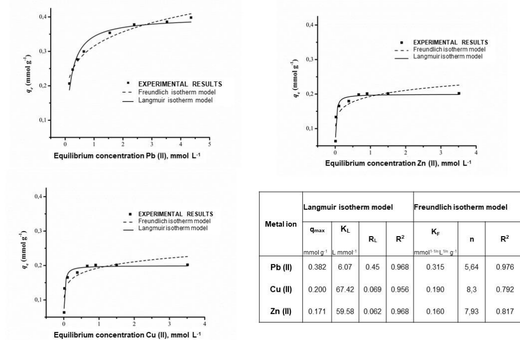
Figure 3. Langmuir and Freundlich isotherm models for Pb(II), Cu(II) and Zn(II) ion biosorption on the CS
