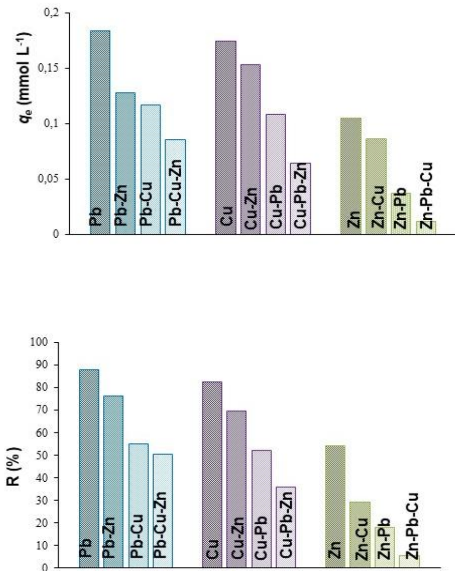
Figure 4. Mutual impact of Pb(II), Cu(II) and Zn(II) ions on the biosorption performance of the CS
