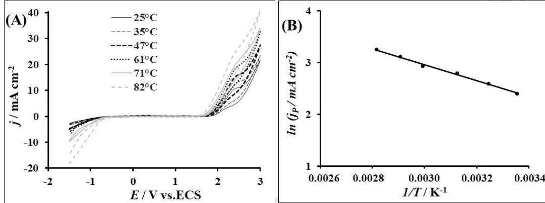
Figure 4. A) Cyclic voltammetry curves recorded on BDD electrode at several temperatures in 0.1 M H 2 SO 4 containing 3,2 mM IOX under the potential scan rate: 50 mV/s, (B) plot of \ln j_p = f(1/T)
