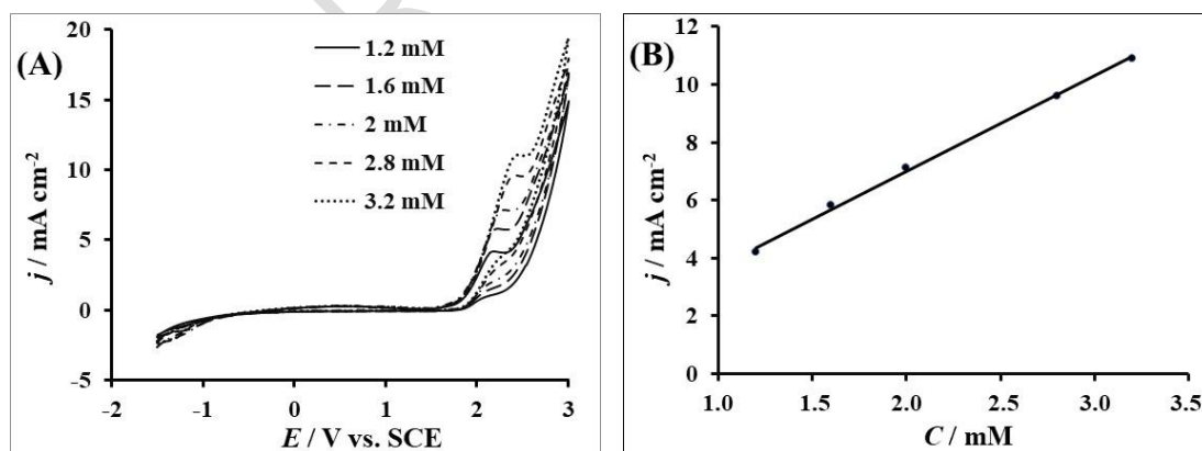
Figure 2. (A) Cyclic voltammetry curves recorded on the BDD in H 2 SO 4 (0.1M) in the presence of different IOX concentrations at 50 mV / s; (B) plot of current density of the IOX oxidation peak versus IOX concentrations.
