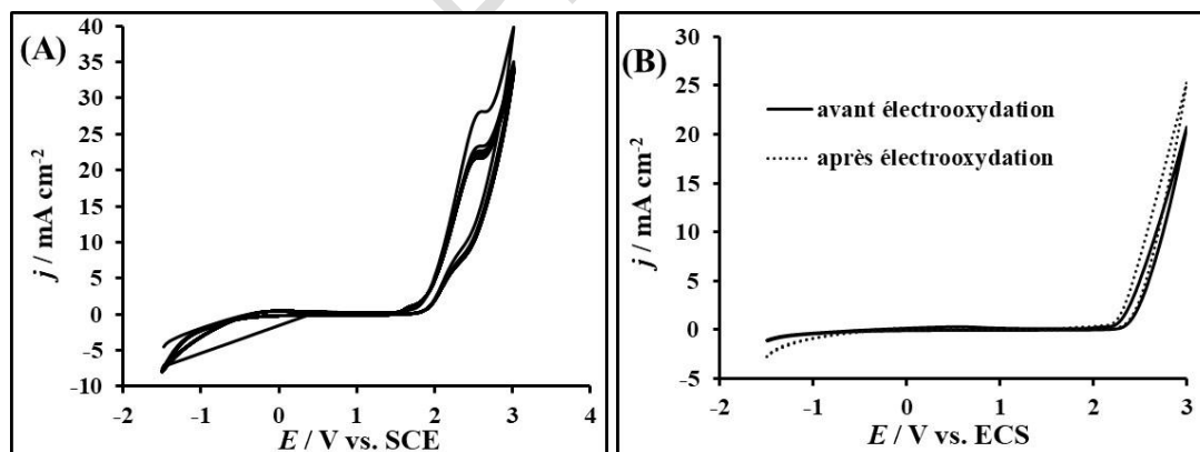
Figure 3: (A) Cyclic voltammogram of BDD in 0.1 M \text{H}_2\text{SO}_4 for 23 successive Cycles in scans performed; (B) Cyclic voltammogram of BDD in 0.1 M \text{H}_2\text{SO}_4 before and after electrooxidation.
