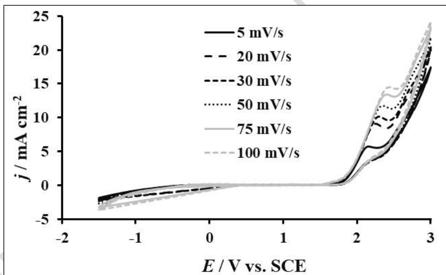
Figure 5: Cyclic voltammograms recorded on BDD electrodes in 3,2 mM IOX containing in 0.1 M H_2SO_4 at several potential scan rates (5-100 mV/s).
