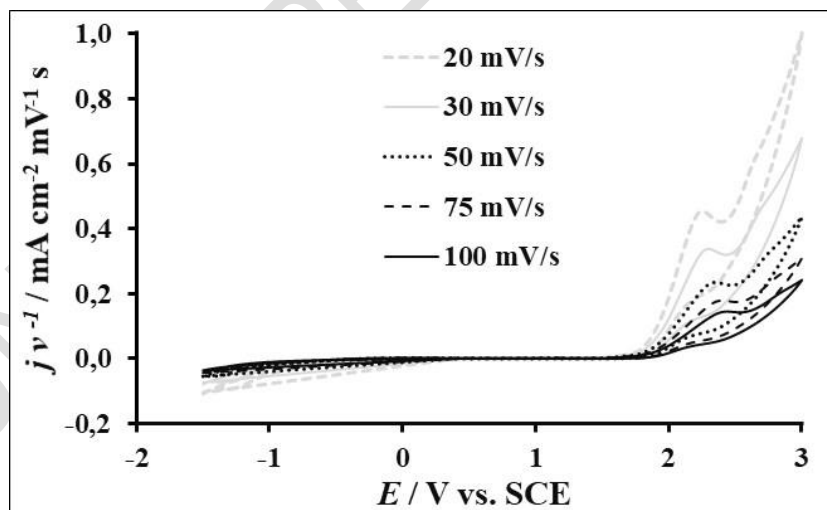
Figure 8: Normalized current density of the cyclic voltammetry measurement recorded on (A) BDD in 0.1 M H_2SO_4 containing 3,2 mM IOX with the potential scan rates (20-100 mV/s) versus applied potential
