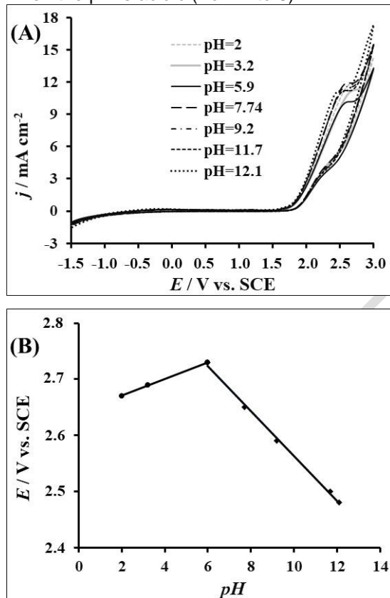
Figure 9: (A) Cyclic voltammograms recorded on BDD at different pH in H 2 SO 4 (0.1M) containing 3.2mM of IOX at 50mV / s; (B) Peak potential as a function of pH
