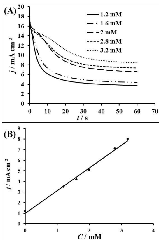
Figure 11: (A) Chronoamperogram of BDD in H 2 SO 4 (0.1M) pH=9 media with several concentrations of IOX. Applied potential E=2.4 V /ECS; (B) Current density versus IOX concentration curve.
