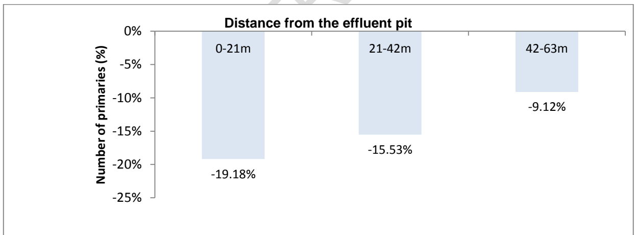
Fig 4 : Graphical representation of decreased number of primaries over control influenced by distance from the effluent pit
