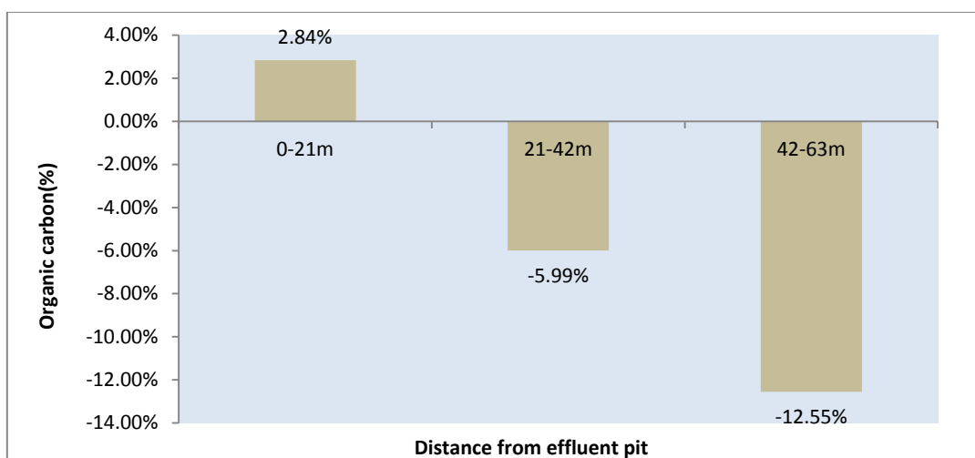
Fig. 9: Graphical representation of percentage increase/decrease organic carbon (%) over control influenced by distance from effluent pit
