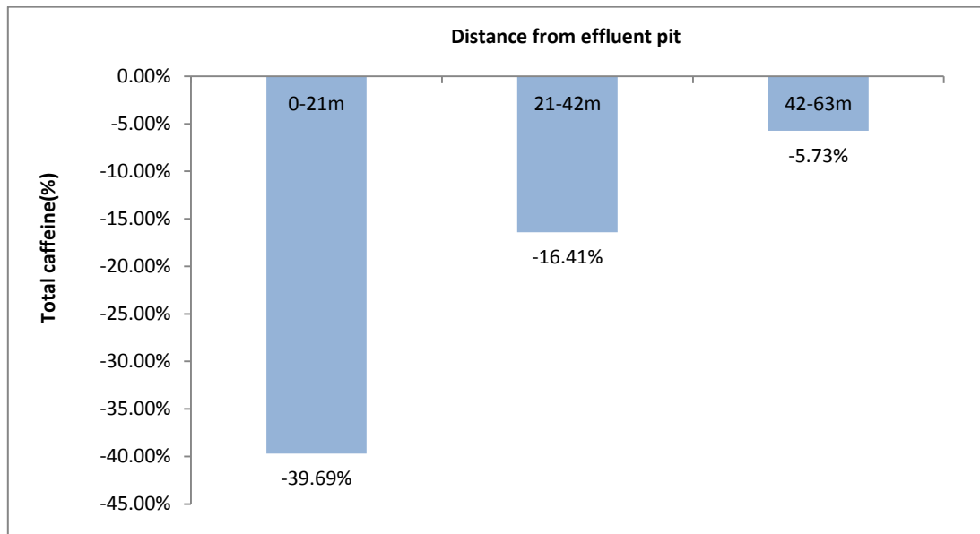
Fig 1: Graphical representation of percentage decrease of total caffeine (%) over control, influenced by distance
