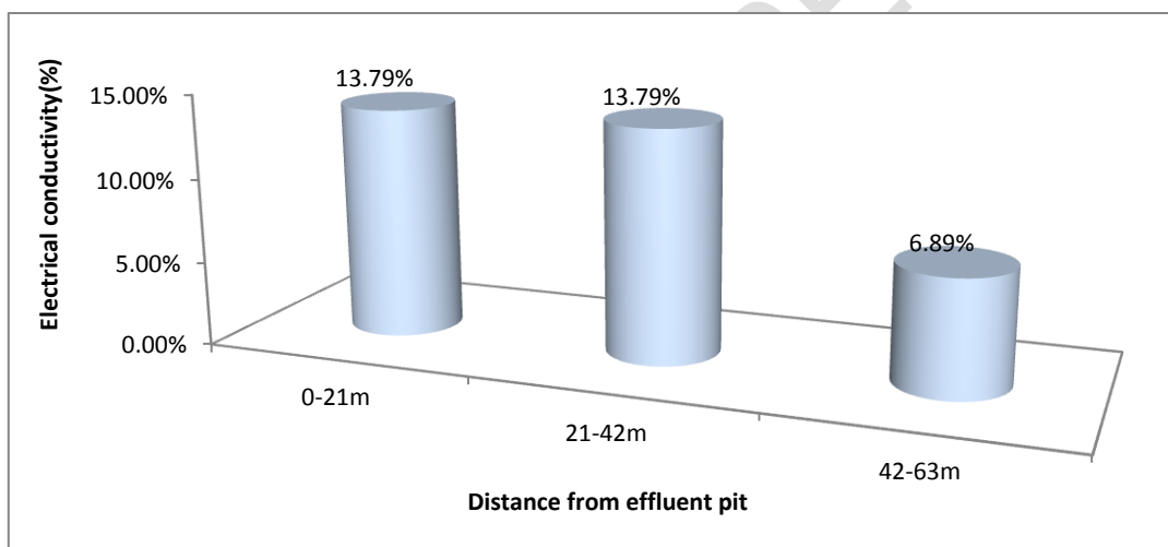
Fig. 10: Graphical representation of percentage increase of electrical conductivity (%) over control influenced by distance from effluent pit
