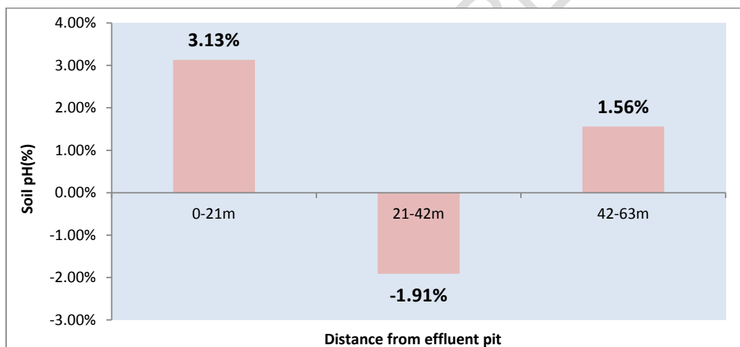
Fig 8 : Graphical representation of decreased or increased soil pH (%) over control influenced by distance from the effluent pit
