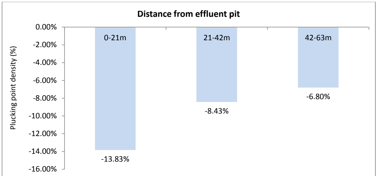
Fig 3 : Graphical representation of percentage decrease plucking point density over control influenced by distance from the effluent pit
