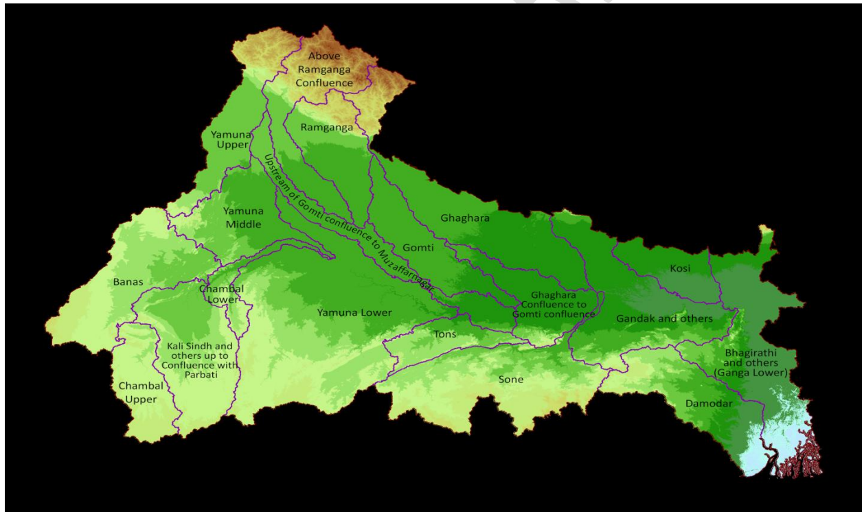
Fig 4: Elevation Zone
