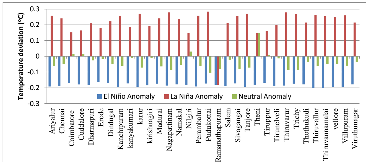
Fig.2. Influence of ENSO on Cold Weather Period (CWP) mean minimum temperature in different districts over Tamil Nadu (1971 - 2013)
