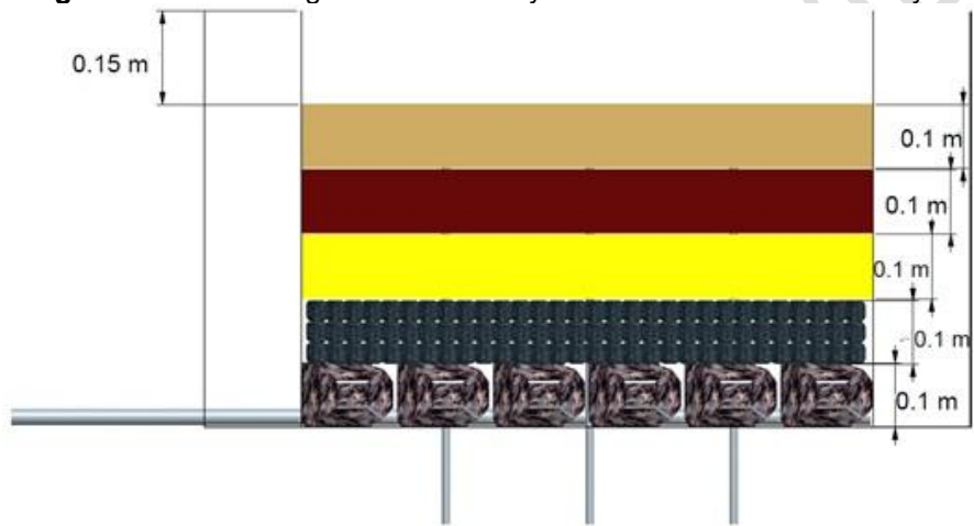
Fig. 6. Thickness of the each layer in laboratory scale constructed wetland system
