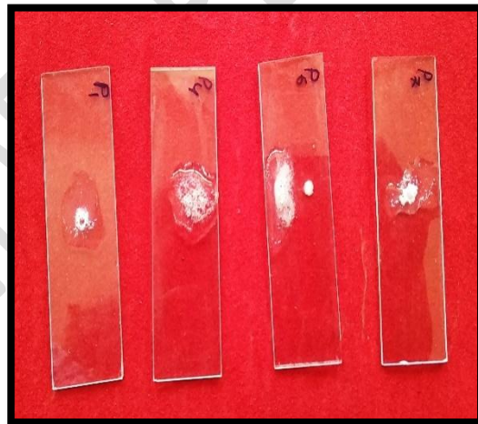
Figure 3: Catalase test
