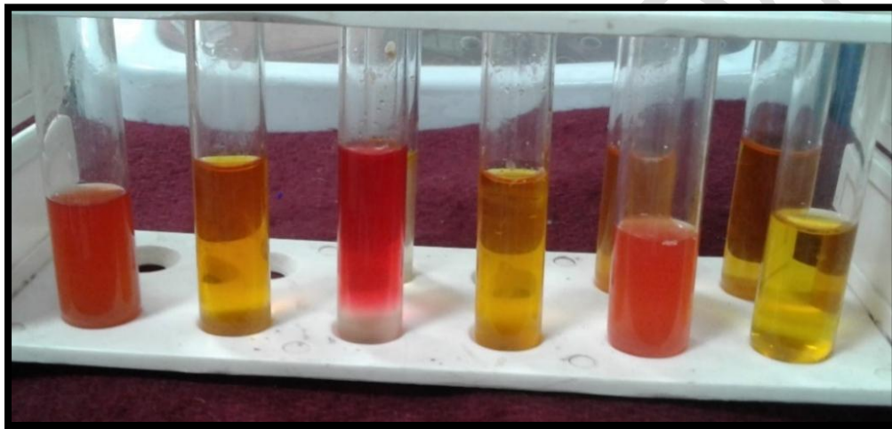
Figure 5: Methyl red test
