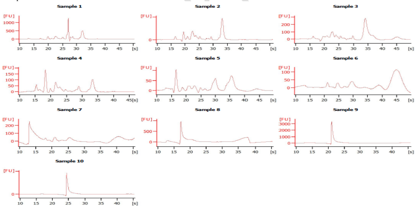
Electrophoresis Plate 3
