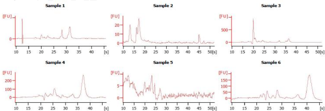
Electrophoresis Plate 5
