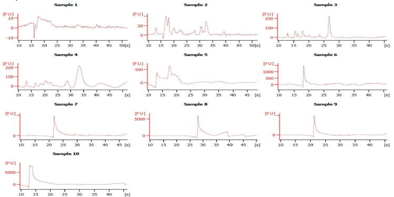
Electrophoresis Plate 2
