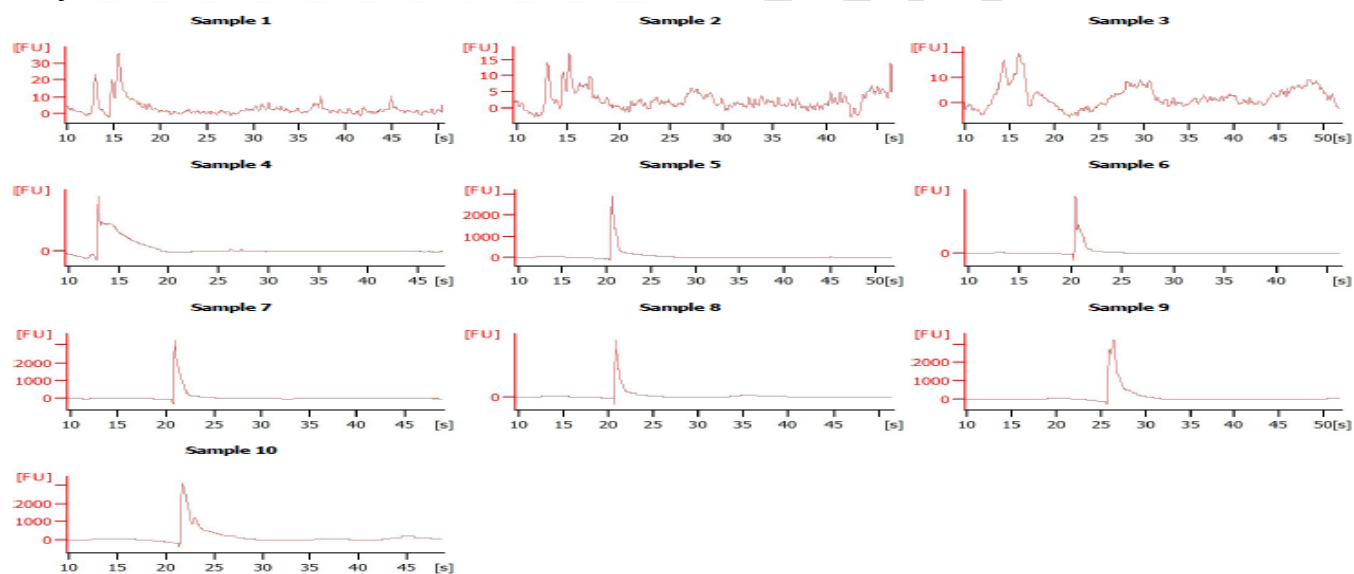
Electrophoresis Plate 5
