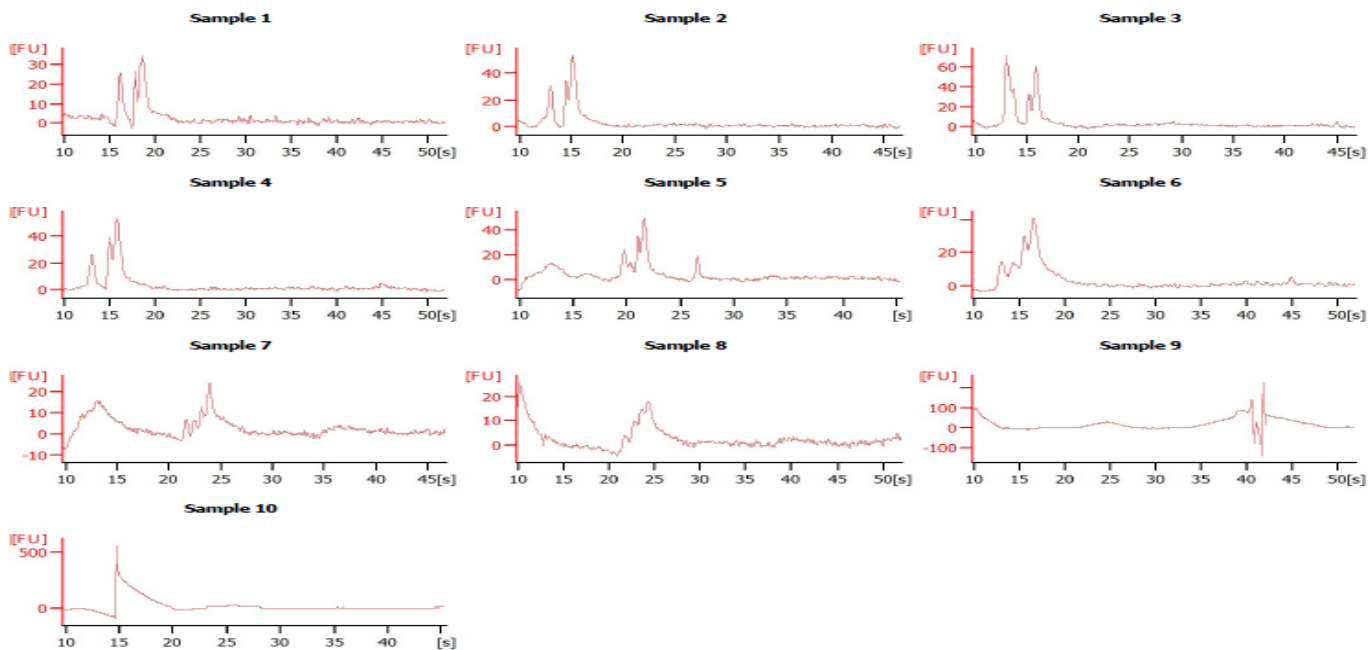
Electrophoresis Plate 4
