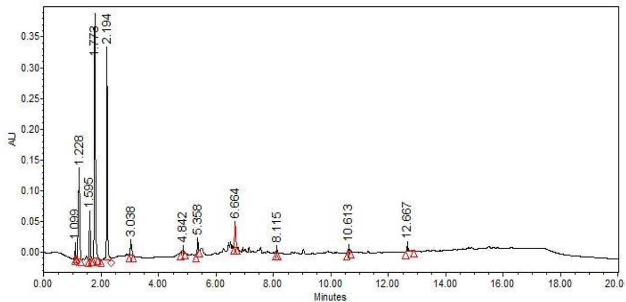
Figure 1 LC-MS chromatogram of Mucuna pruriens seed.
