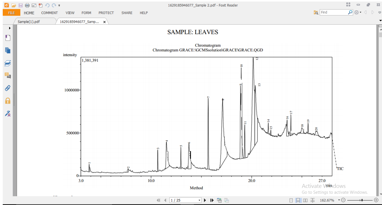
Fig 10. GC-MS chromatogram of M.p leaf
