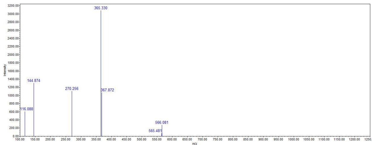
Fig 6 Mass spectrum for Acetylauustoinide ( Diterpenoid) identified in M.p leaf (RT 6.77)
