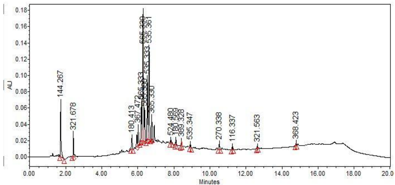
Fig 4 LC-MS MUCUNA P. LEAF CHROMATOGRAM
