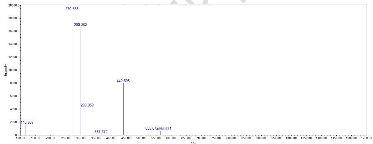
Fig 5 Mass spectrum for Epioxylubianin (Sesquineperoxide) ) identified in M.p leaf (RT 10.52)
