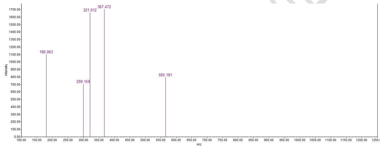
Fig 7 furocoumarine acid glycoside (phenolic glycoside) identified in M.p leaf (RT 6.02)
