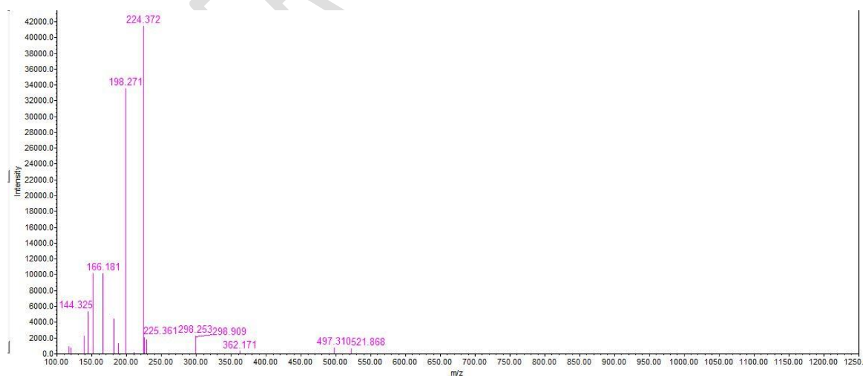
Figure 2 Hydroxystreptozolin ( Oxazolidene) identified in M.p seed (RT 2.19)
