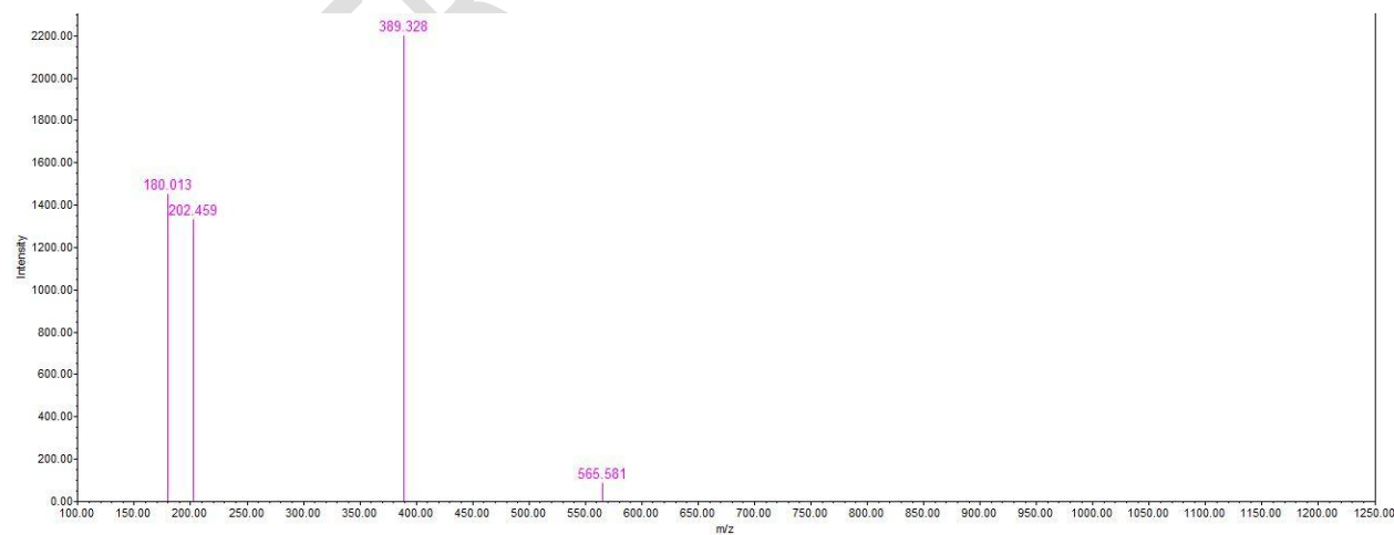
Fig 8. Mass spectrum for Quassin (Quaesinoids) identified in M.p leaf (RT 8.41)
