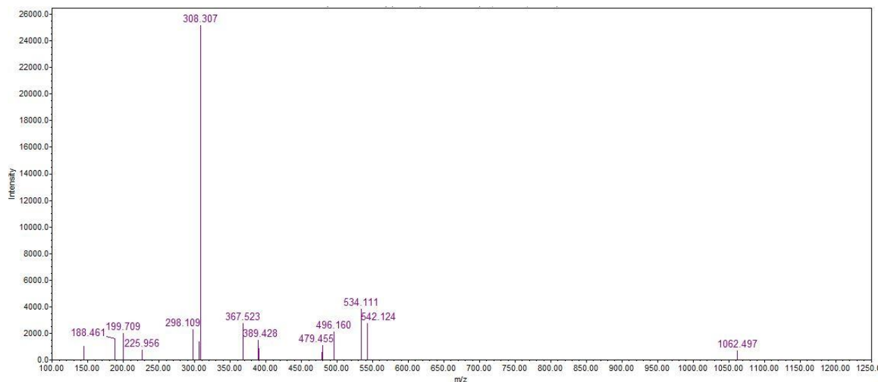
Figure 3: Dihydrocapsaicin (Meltocypenol) identified in M.p seed ( RT 12.66)
