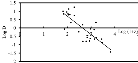
Figure 2: The scatter plot of linear size against redshift for CSS galaxies
