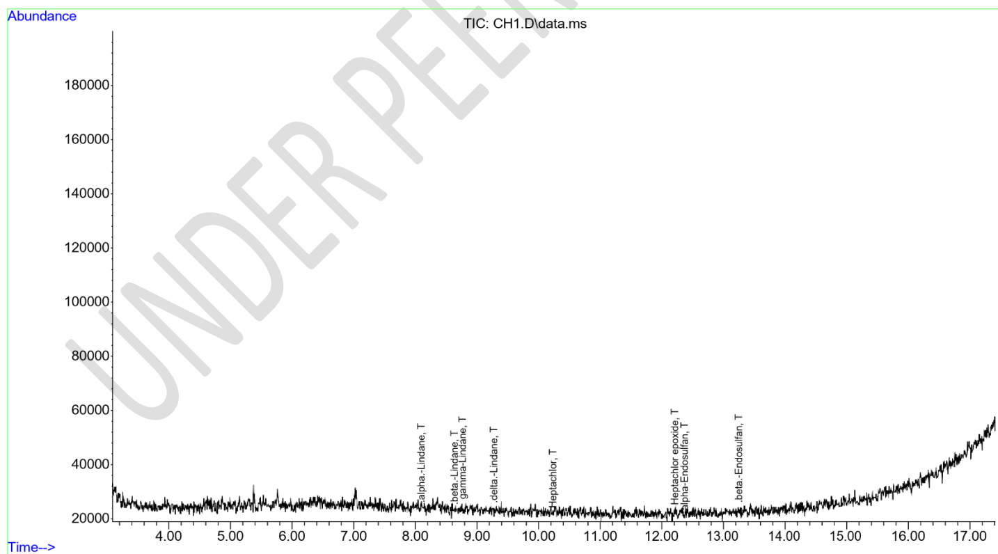
GC-MS CHROMAMATOGRAM FOR THE STREAM SAMPLE OF AD 2 GC-MS CHROMAMATOGRAM FOR THE STREAM SAMPLE OF CH 1
