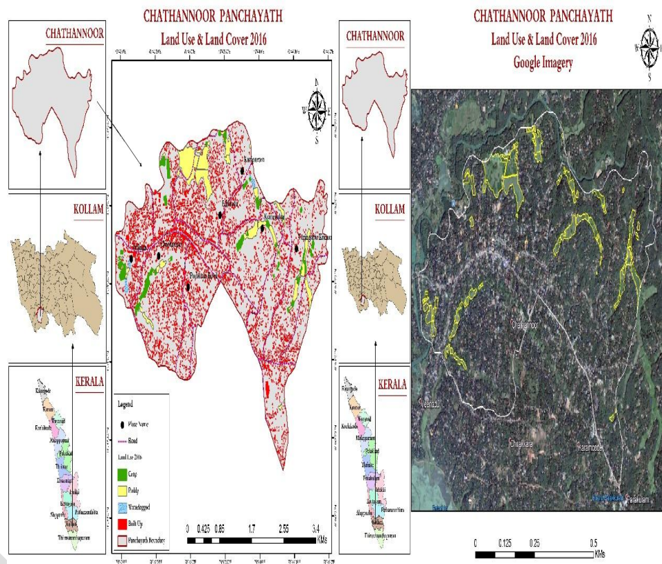
Fig. 6. Distribution of LULC variables in 2016.
