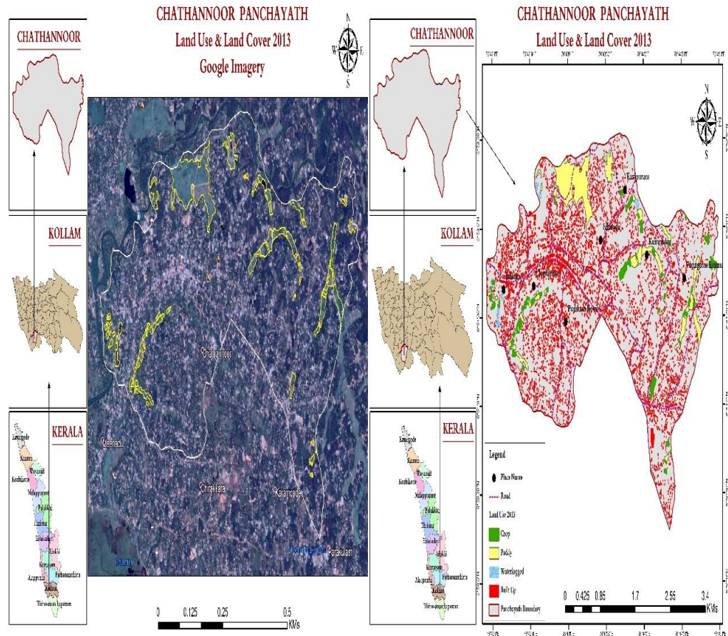
Fig. 5. Distribution of LULC variables in 2013.
