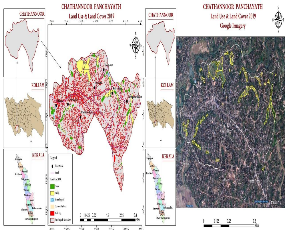
Fig. 7. Distribution of LULC variables in 2019.
