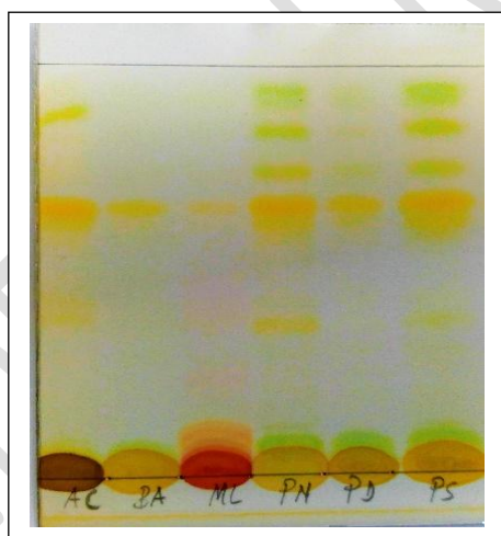
Figure 9. Chromatogram for alkaloids [Mobile phase: Toluene/ethyl acetate/diethylamine (35: 10: 5); Detection: NaNO 2 5%]. Alkaloids are characterized by the presence of orange
