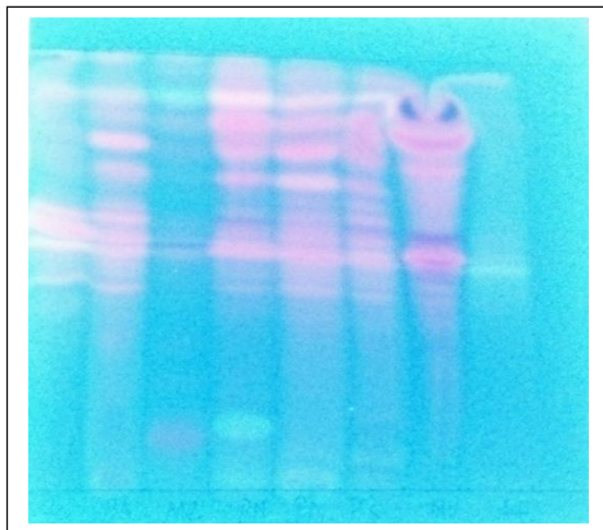
Figure 11. Chromatogram of the methanolic extract of A. cordifolia , B. alba , M. lucida , P. nigrescens , P. dodecandra and P. scandens for anthraquinones; Mobile phase: Ethyl acetate/Methanol/Water (50: 8.5: 6.5). Detection: by UV light at 366 nm.
