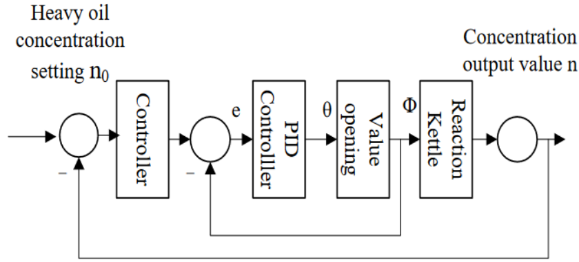
Figure 7 Control principle of the gasoline concentration. [59]
