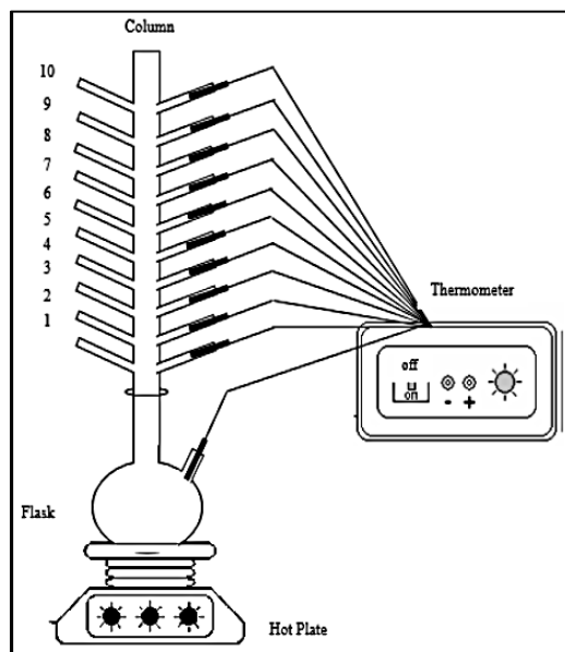
Fig.1. schematic diagram of the thermal distillation
