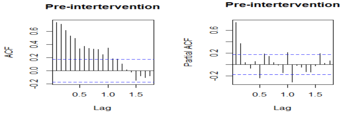
Fig.3: ACF and PACF Plots of Pre-intervention
