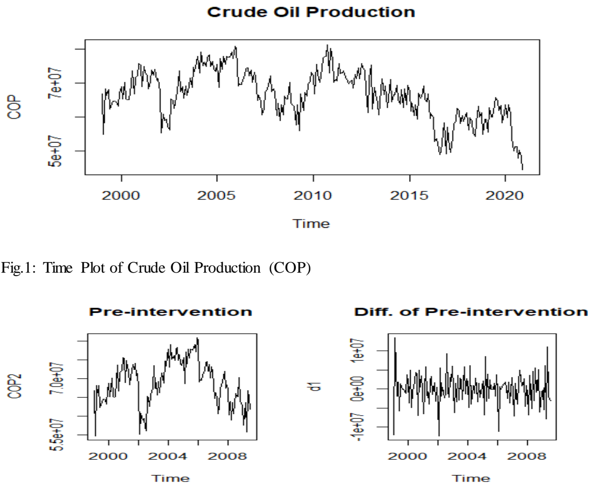
Fig.2: Time Plot of Pre-intervention Series before and after First Difference
