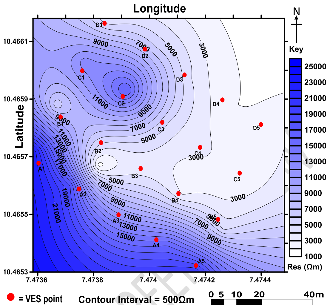
Fig 8: Transverse Resistance Map of the Study Area
