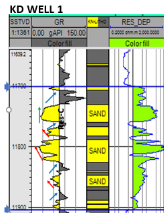
Log Shape Type
