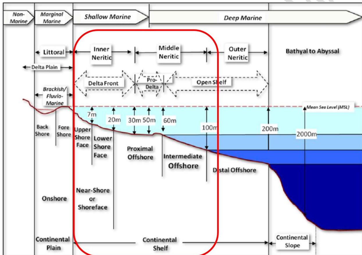
Figure 9: Depositional environments and bathymetric ranges used for palaeoenvironmental interpretation [21], showing the environment of deposition for KD FIELD within the red line.
