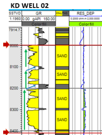
Log Shape Type
