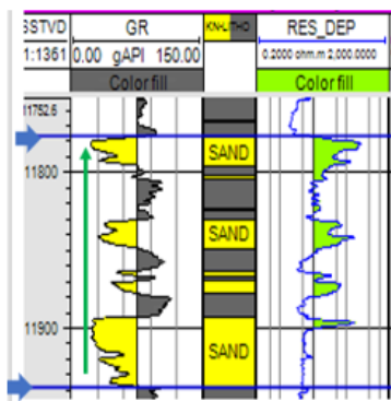
Figure 8: Parasequence and Delineation of Environment of deposition using Log Motif for KD 03 well (Reservoir-C)
