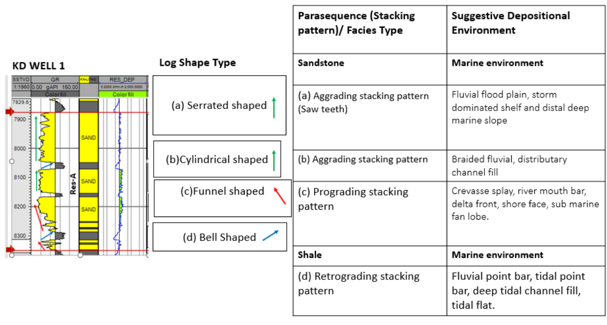
Figure 2: Parasequence and environment of deposition using Log Motif of KD 01 well (Reservoir A)
