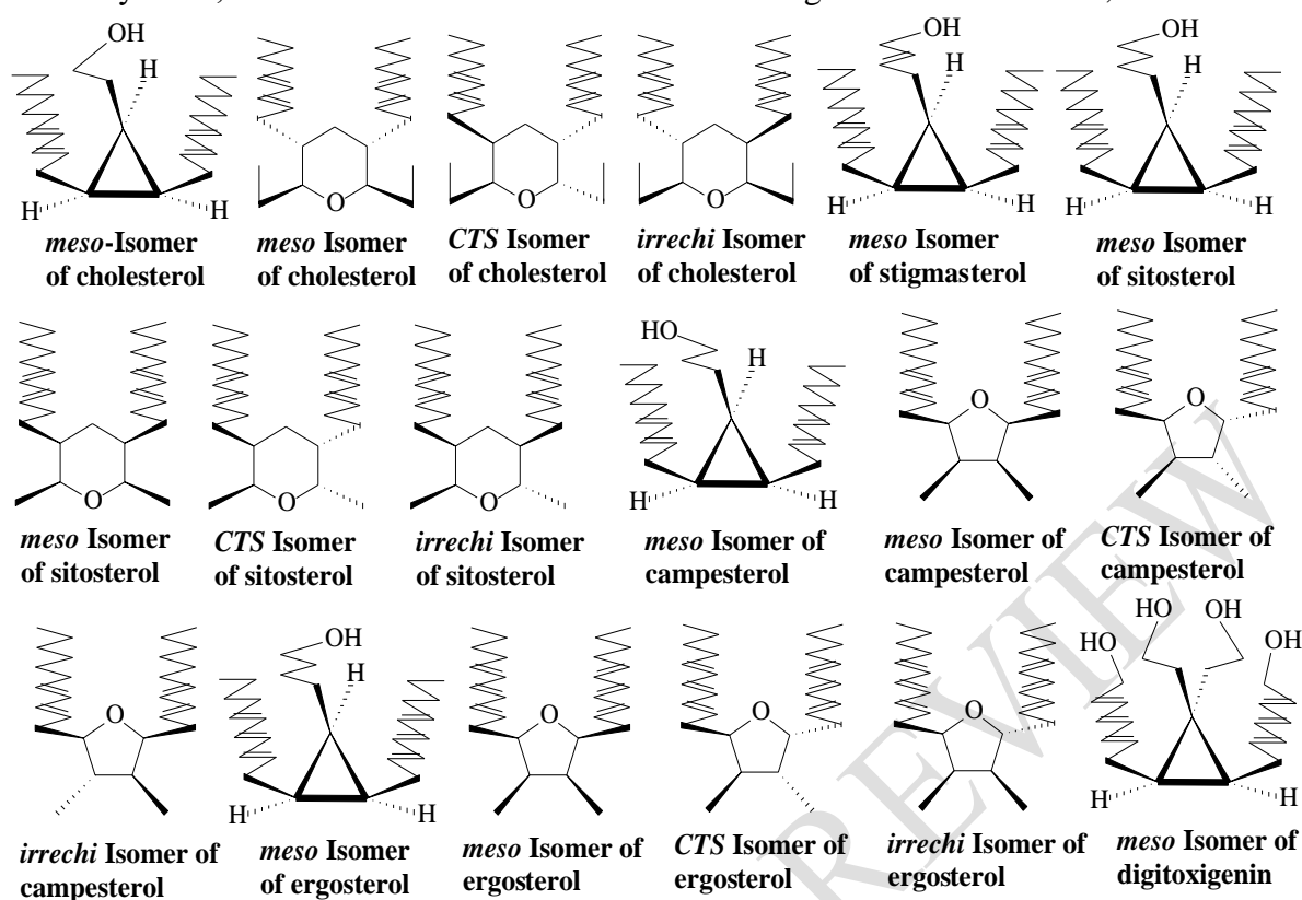
Figure 9. Meso isomers of some natural sterols.
