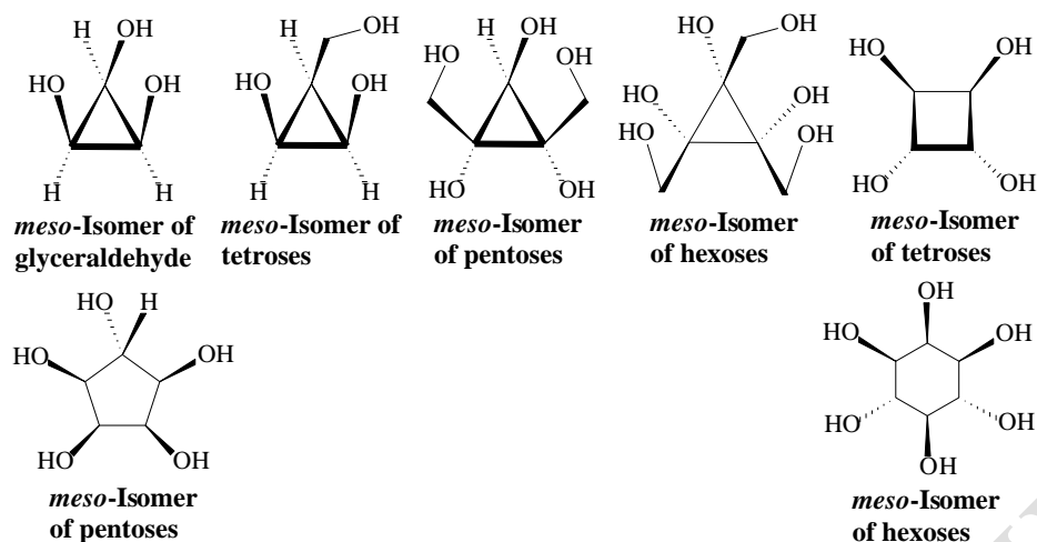
Figure 6. Meso isomers of aldoses and ketoses.
