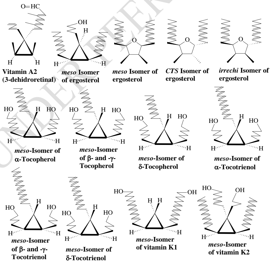
Figure 9. Meso isomers of some natural sterols.
