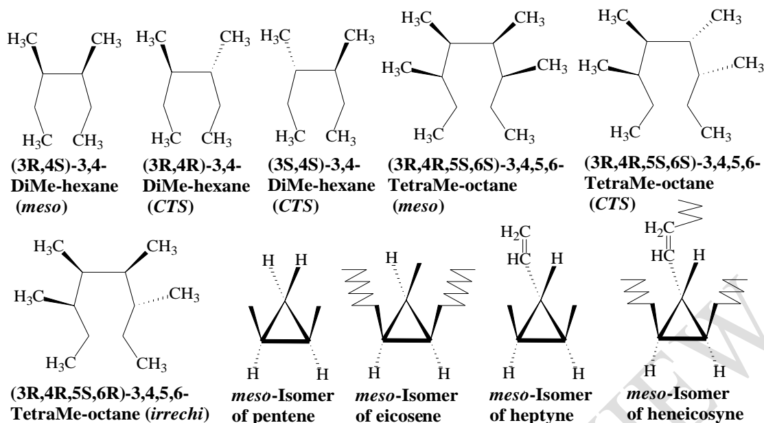
Figure 2. Meso isomers of saturated and unsaturated hydrocarbons.
