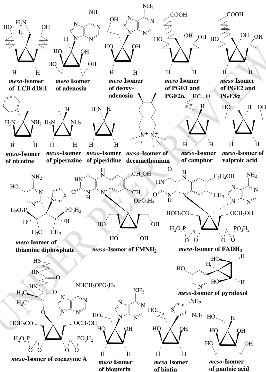
Figure 8. Meso isomers of some natural compounds, including hydrosoluble vitamins.
