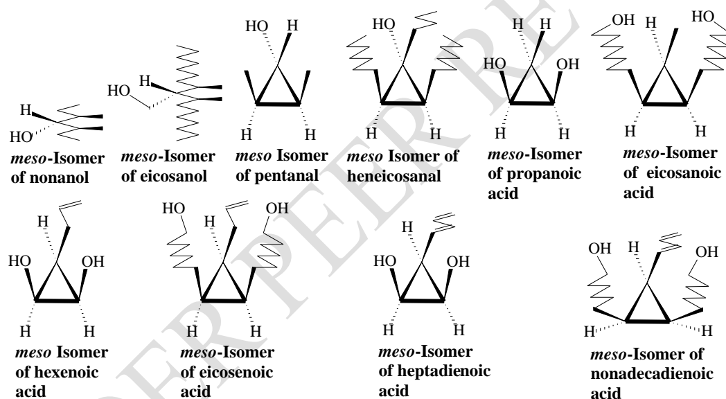
Figure 3. Meso isomers of some serial compounds with functional groups.
