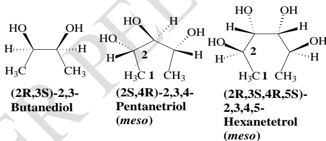
Figure 4. Meso isomers of some epoxides.
