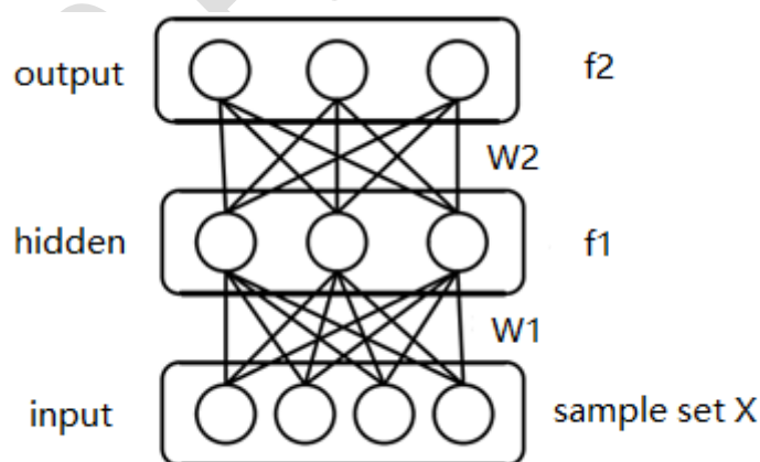
Figure 2 Three-layer neural network structure of sparse filtering model
