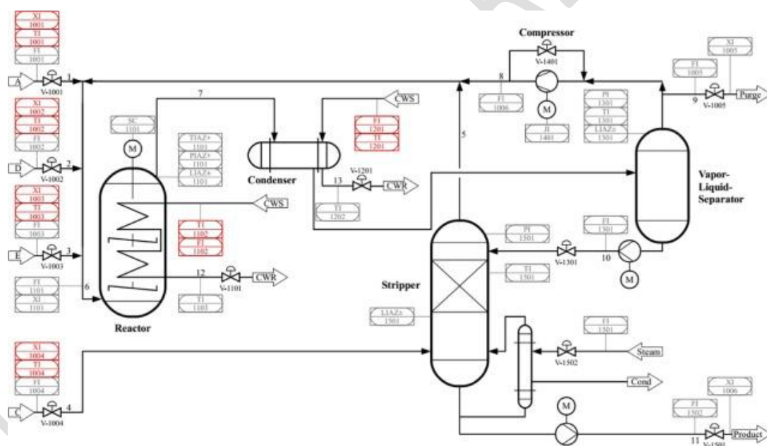
Figure 3 Process flow diagram of TE process
