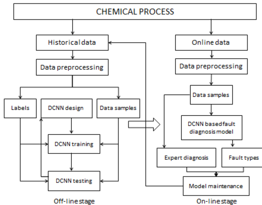
Figure 4 The framework of the DCNN based fault diagnosis method
