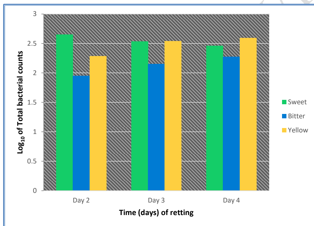
Figure 1a: \text{Log}_{10} of the total bacterial counts per days of retting
