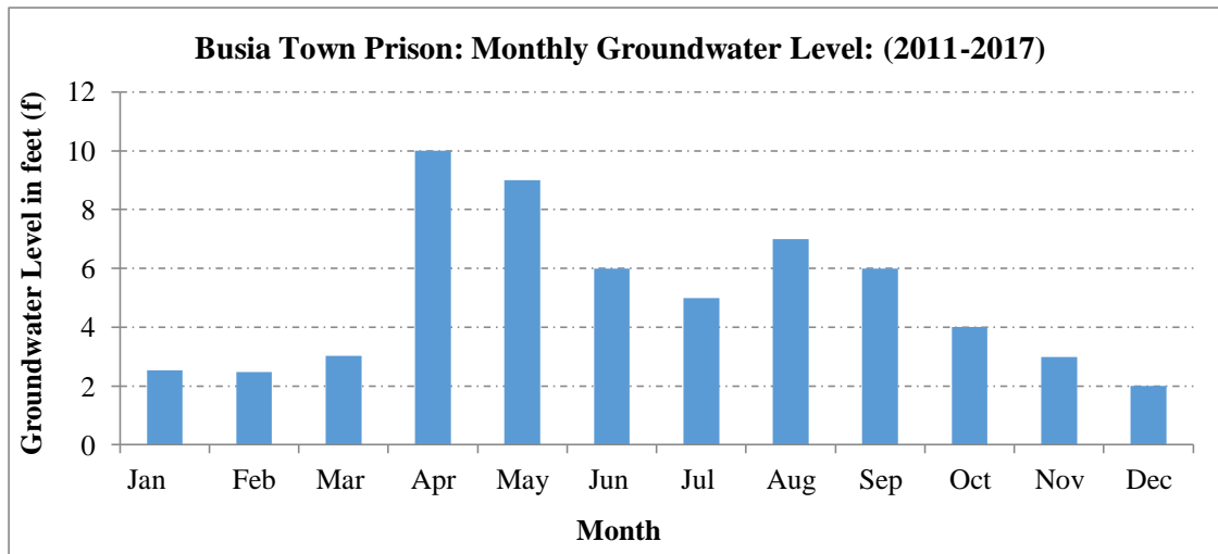
Figure 4: Kakamega Mwikalikha School, Kakamega Tande School, Bungoma Water Supply and Busia Town Prison monthly mean groundwater levels compared with Kakamega meteorological station monthly mean minimum, maximum and mean temperatures.
