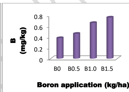
Fig. 2 Effect of boron on B (mg/kg)
