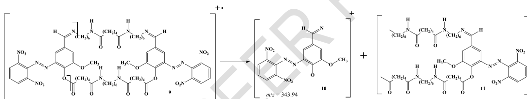
Figure 2: The fragment M^+ - 991.48 of amide 9 .
