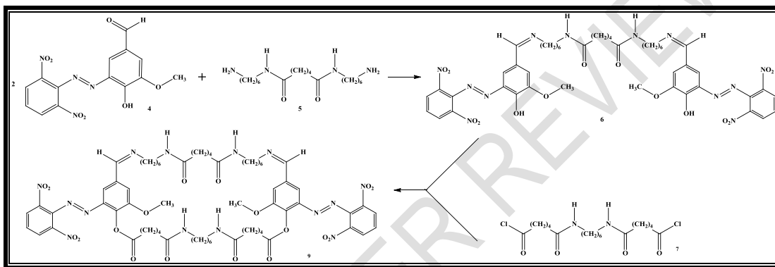
Scheme 3: The first pathway for synthesis of 9 .
