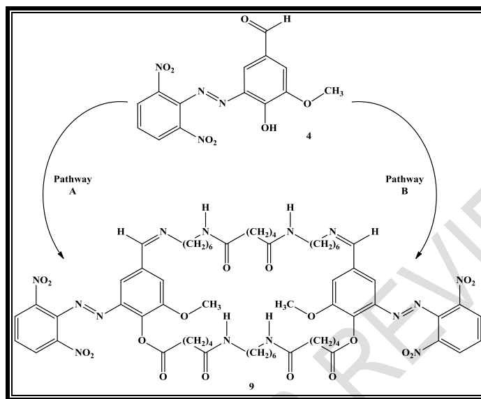
Scheme 1: The new synthesized of amide 9
