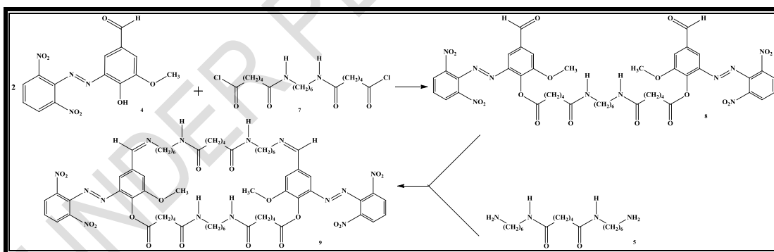
Scheme 3: The first pathway for synthesis of 9 .
