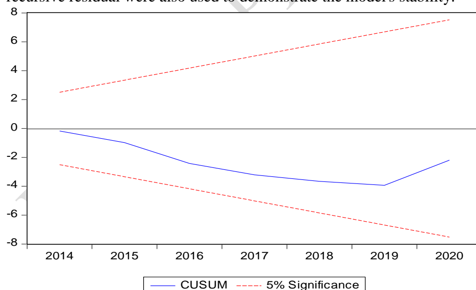
Fig 1: Stability model
