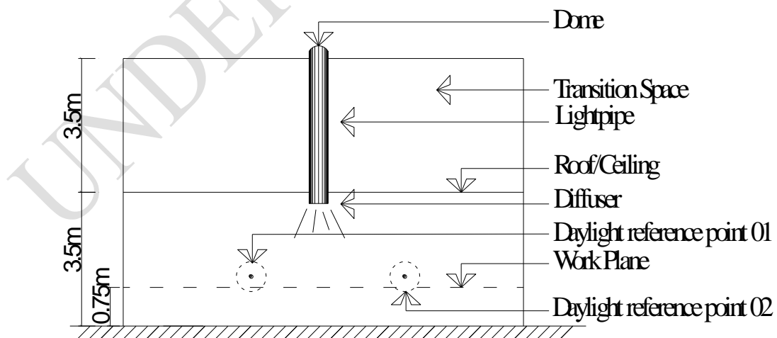
Figure 4. Light pipe and daylight reference points (section)
