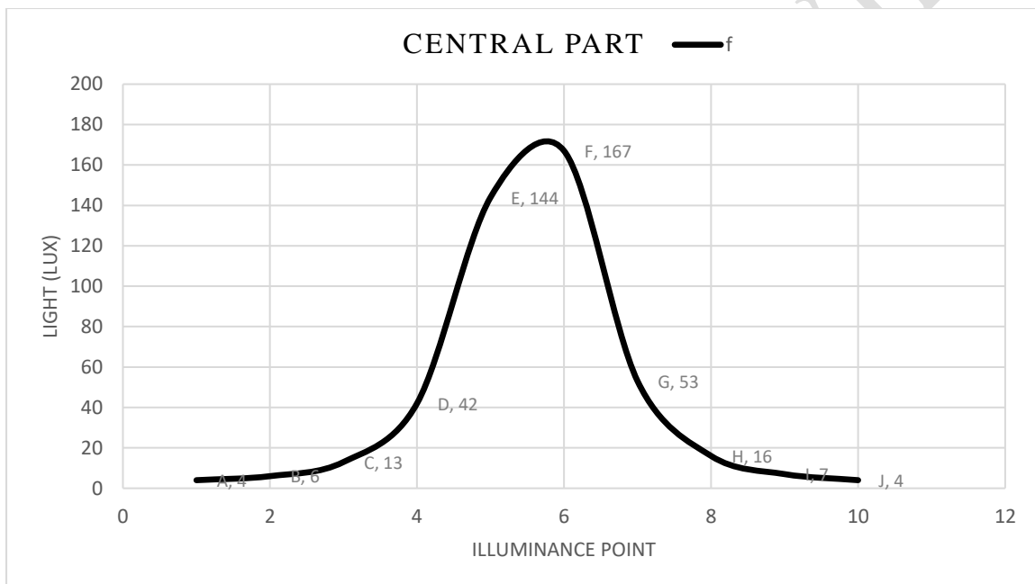
Figure 9. Daylighting distribution at central part (f) for case 01(b)
