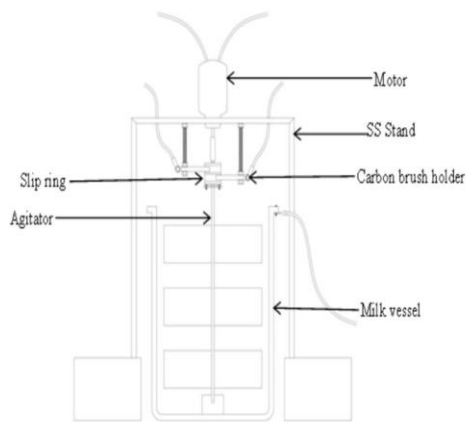
Figure 1: The conceptual diagram of an ohmic heater
