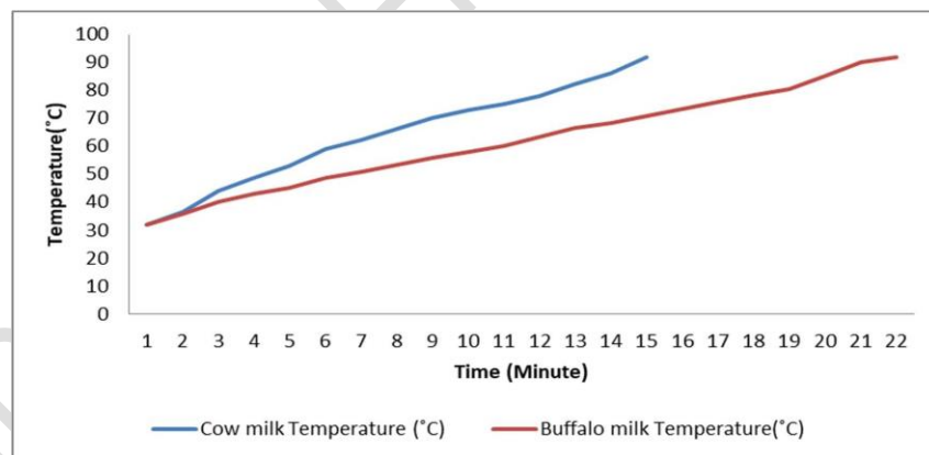
Figure 4: Temperature profile during ohmic heating
