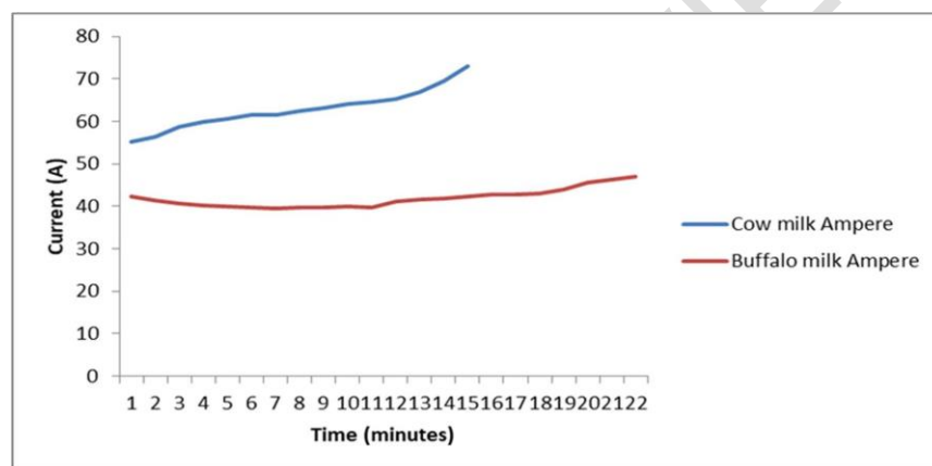
Figure 5: Current profile during ohmic heating
