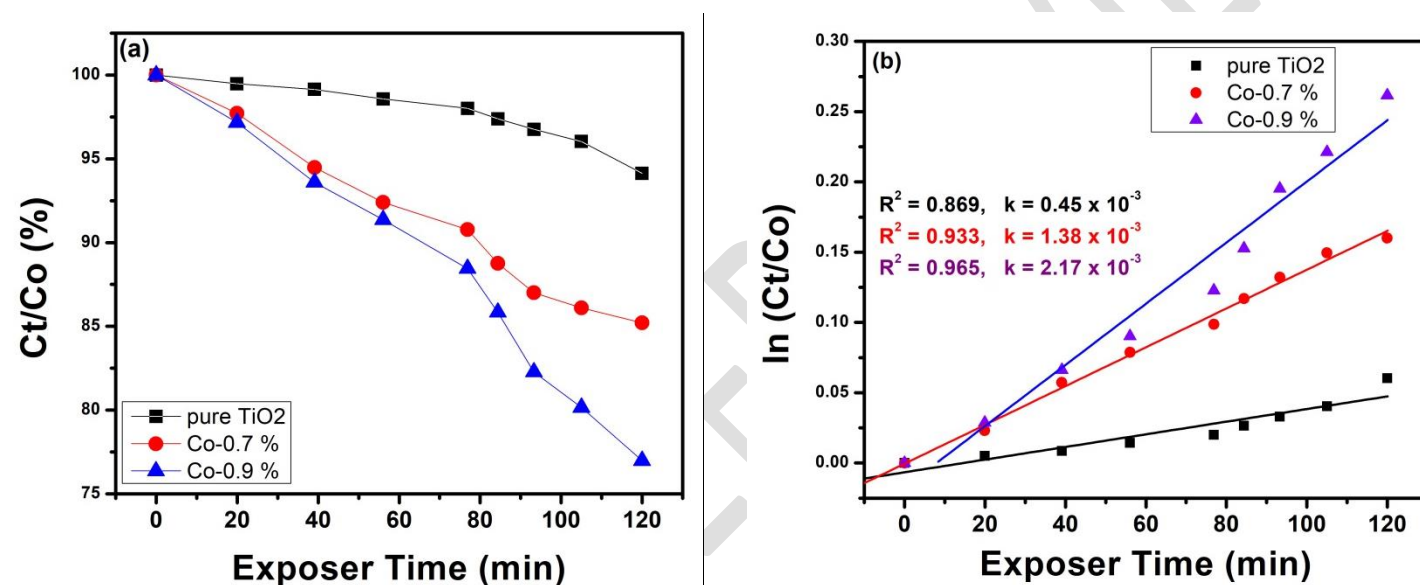
Figure 6. Pseudo First-order model reaction kinetics (a) C_t/C_0 %, (b) \ln(C_t/C_0) pure, 0.7 % and 0.9 % Co-doped \text{TiO}_2 nano-photocatalysts
