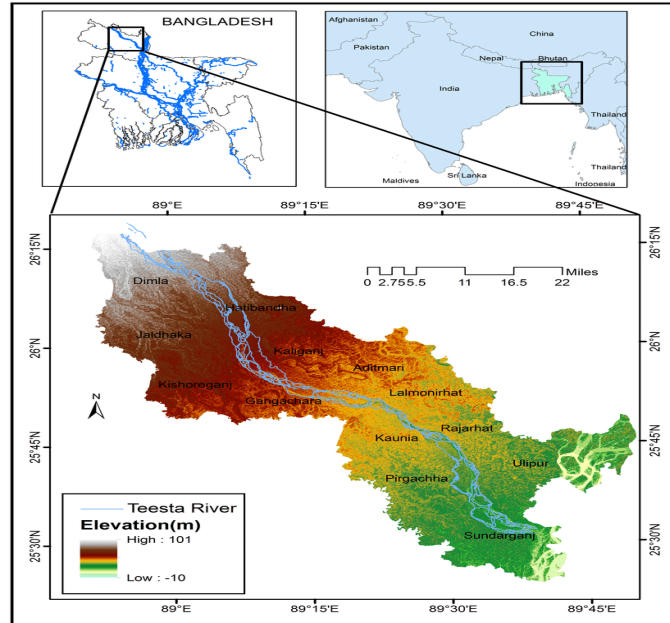
Fig.1. Teesta Watershed [19]
