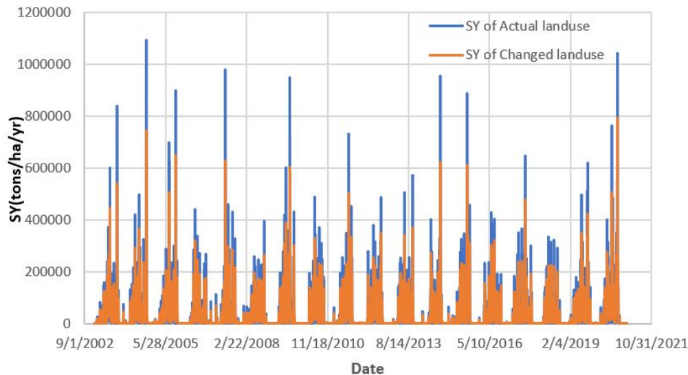
Fig. 10. Simulated sediment for two different types of land use
