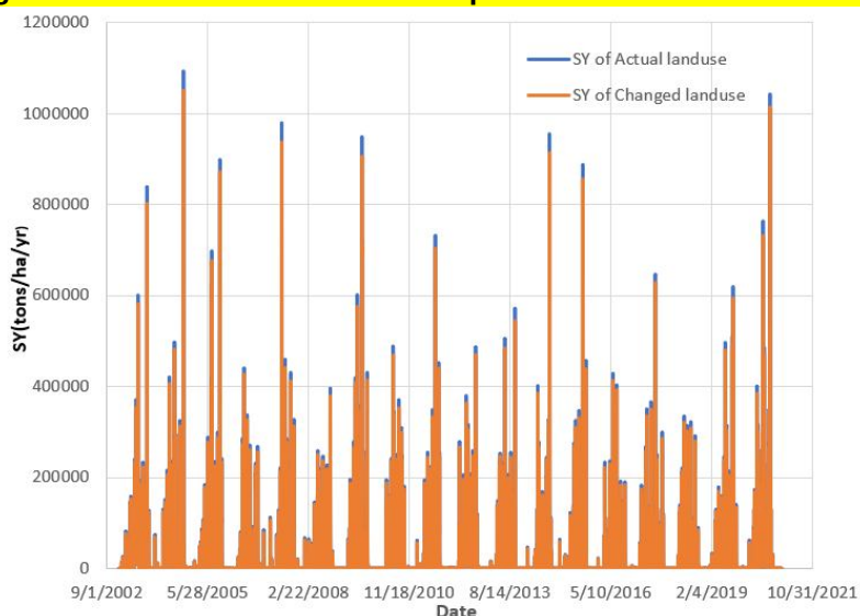
Fig. 14. Simulated sediment for two different types of land use
