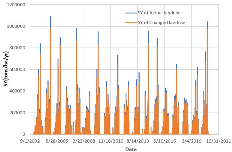
Fig. 8: Simulated sediment for two different types of land use
