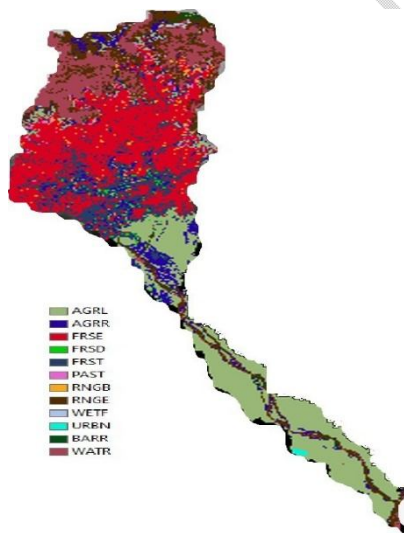
Fig. 3. Land use and land cover map of the Teesta River Catchment
