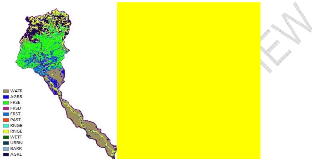
Fig. 7. Land use and land cover map of the Teesta River Catchment
