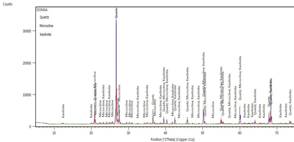
Figure 4: XRD MEASUREMENT FOR DONGA SOILS
