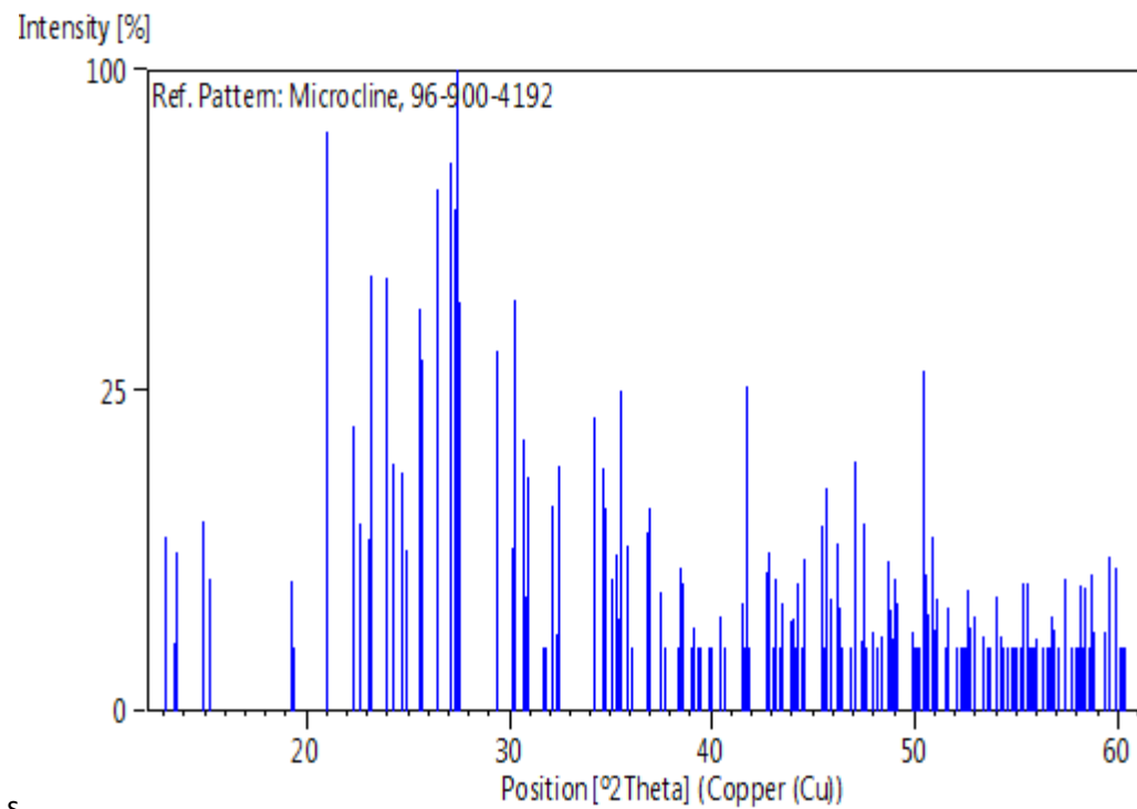
s Figure 6: Stick Pattern showing peaks of Microcline in clay samples
